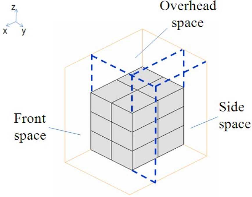
Figure 10: Split Space.
