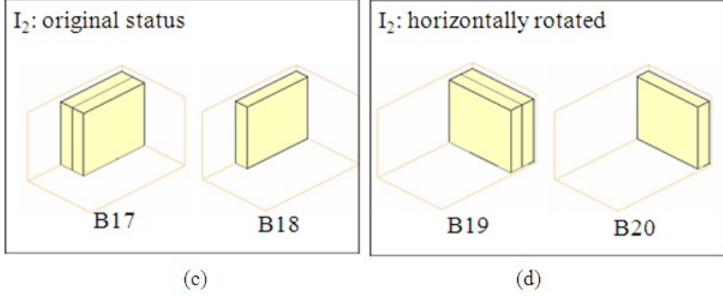
Figure 7: Possible Blocks.
