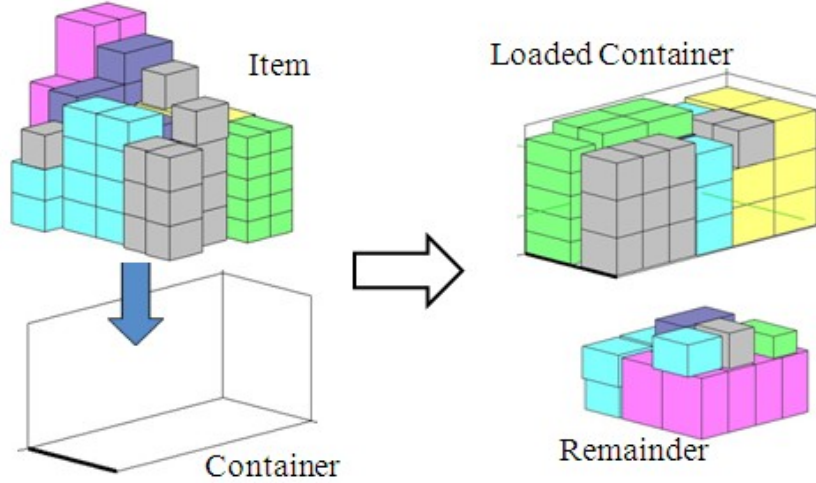
Figure 1: The CLP.
