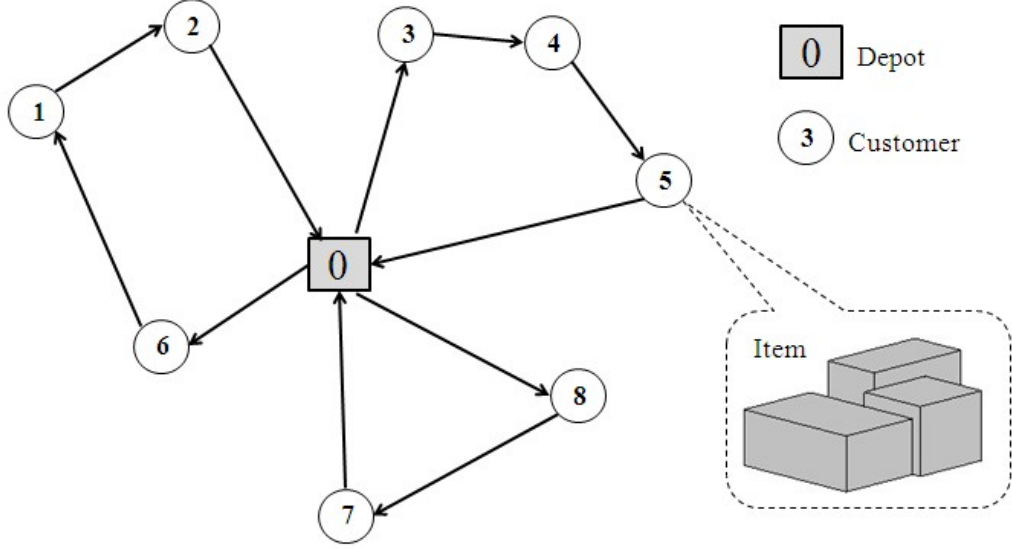
Figure 2: The 3L-CVRP.
