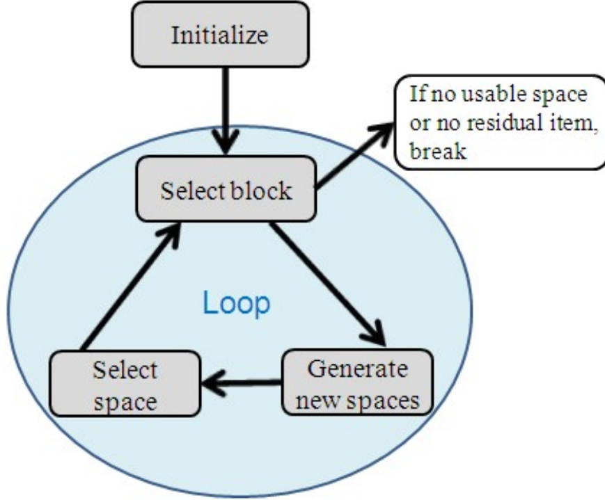
Figure 9: Algorithm HEUR_SCLP.
