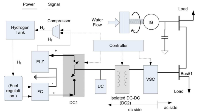
Fig. 1. Layout of the proposed system.
