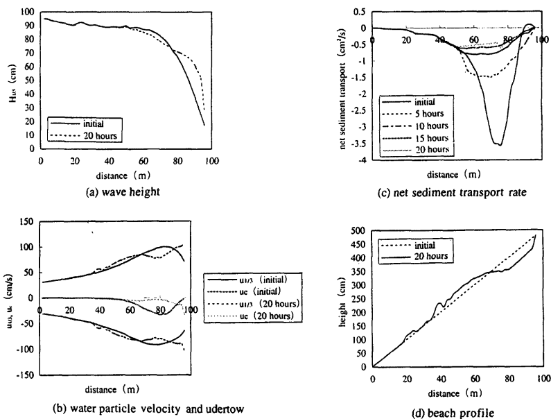
Fig.10 Simulation results ( Ho/Lo = 0.053 , d = 0.3\text{mm} )
