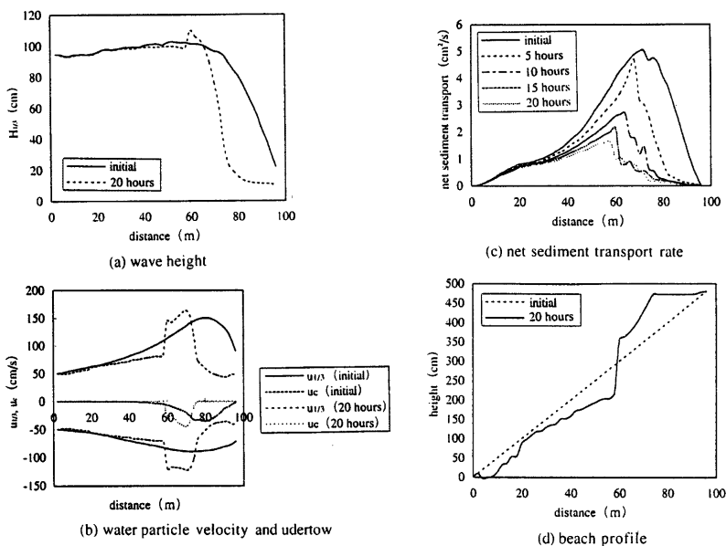
Fig.12 Simulation results ( Ho/Lo=0.022 , d=0.3\text{mm} )
