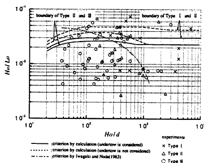
Fig.16 Criterion of beach profiles with the parameter Hold
