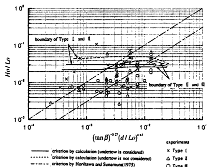
Fig.17 Criterion of beach profiles with the parameter (\tan \beta)^{-0.27}(d/Lo)^{0.67}
