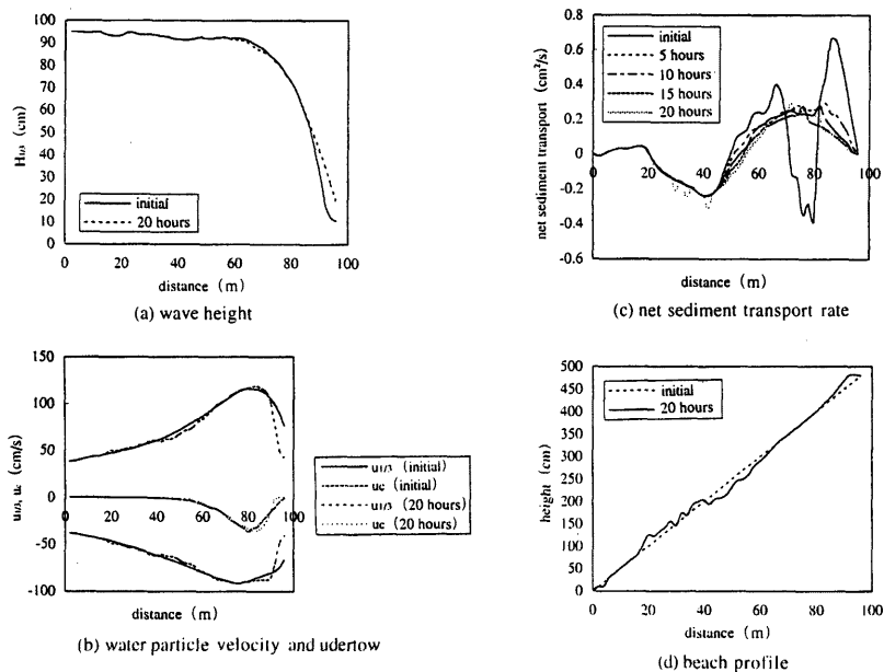
Fig.11 Simulation results ( Ho/Lo = 0.040 , d = 0.3\text{mm} )
