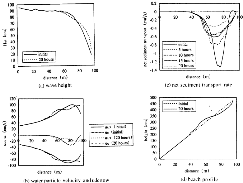
Fig.13 Simulation results ( Ho/Lo=0.053 , d=0.3\text{mm} )
