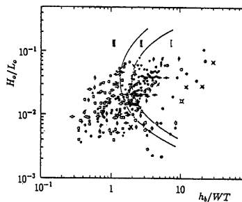
Fig.9 Criterion of beach profile types, from Kawata et al.(1992)
