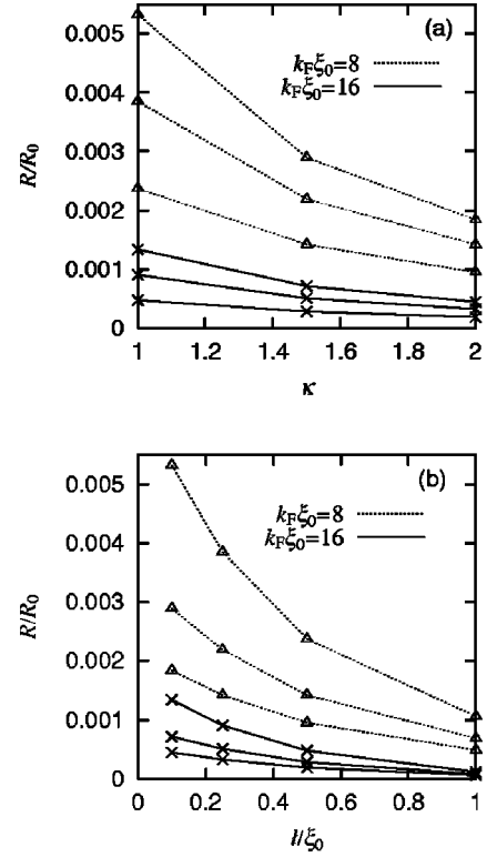
FIG. 3. (a) \kappa dependence of the Hall resistance. Within the same k_F\xi_0 , the three lines from the top correspond to l=0.1\xi_0 , l=0.25\xi_0 , and l=0.5\xi_0 , respectively. (b) l dependence of the Hall resistance. Within the same k_F\xi_0 , three lines from the top correspond to \kappa=1 , \kappa=1.5 , and \kappa=2 , respectively. In both figures the Hall resistance R is scaled by R_0 = h/2e^2 .
