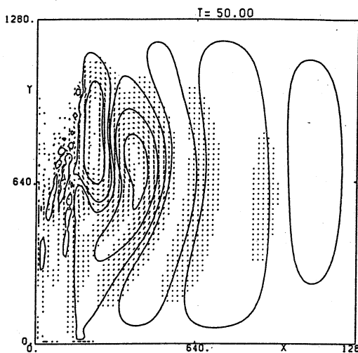
(a) 低気圧性渦
