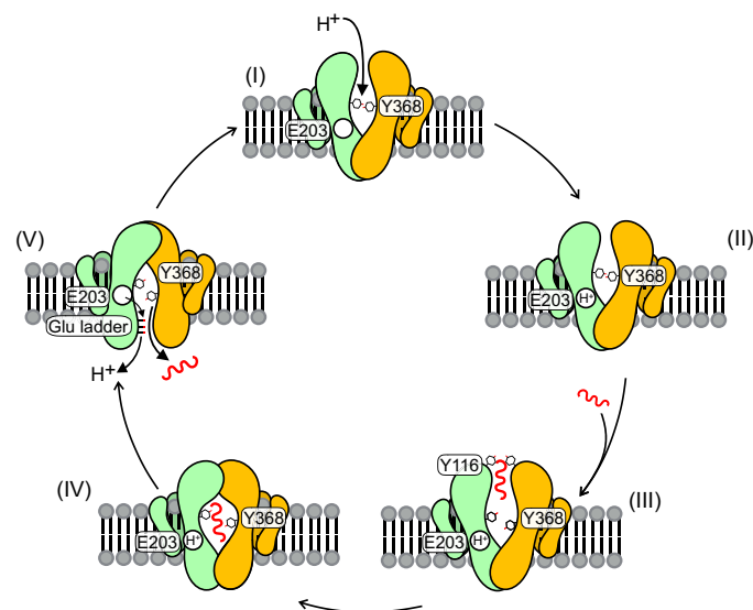
Fig. 4. Proposed mechanism for SbmA peptide transport. (I) Proton is free to bind when the transporter is in the outward-open state, but proton transport is precluded. Inner cavity is occluded by Tyr 368 . Glu 203 is essential for transport and is marked as a potential first proton-binding site (II). (III) Binding of substrate peptide (Tyr 116 is essential for MccB17 and MccJ25) triggers conformational changes, resulting in a transient or stable occluded state (IV). (V) Structural rearrangements result in an inward-open conformation and subsequent release of the proton into the cytoplasm, using the glutamate ladder, leading to the dissociation of the peptide; the transporter resets in its outward-open conformation. Only one copy of the glutamate ladder and Glu 203 is shown for clarity.
