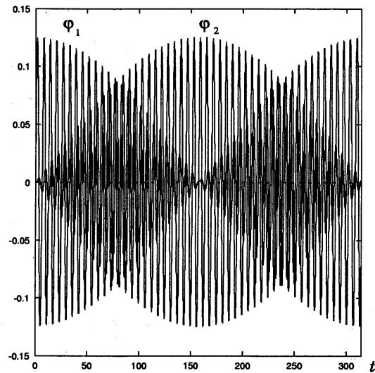
Fig. 3. \varphi_1(t) and \varphi_2(t) on t \in [0, 100\pi] .
