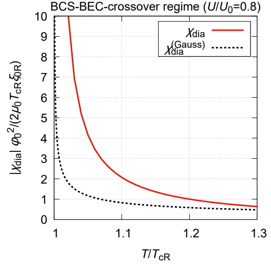
Figure 2.8: SCF-induced diamagnetic susceptibility in the low-field limit as a function of temperature in the BCS-BEC crossover regime. The meaning of lines is the same as in Fig. 2.7.
