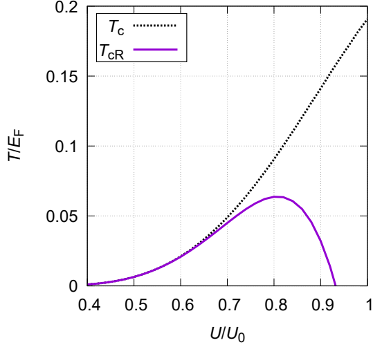
Figure 2.3: The bare critical temperature T_c (black dotted line) and the renormalized critical temperature T_{cR} (purple solid line) as a function of the interaction strength U . Our theoretical approach seems to be valid when U/U_0 \lesssim 0.8 .
