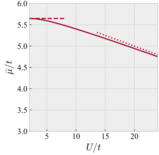
Figure 1.5: Renormalized chemical potential \tilde{\mu} as a function of the attractive interaction U (here \tilde{\mu} is measured from the free-particle band bottom) with high density ( N/M = 0.9 ). The asymptotic forms are also shown in the same way as Fig. 1.3.
