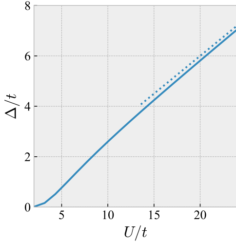
Figure 1.2: Order-parameter amplitude \Delta as a function of the attractive interaction U with low density ( N/M = 0.2 ). The asymptotic form in the BEC regime [Eq. (1.1.18)] is also shown (blue dotted line).
