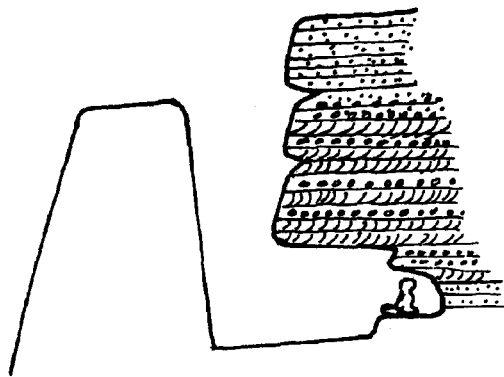
Fig. 23 A Cave Formed through Joint Action of Rock Dislocation and Corrosion, at Wat Tham Khon Pheng along HWY 210
