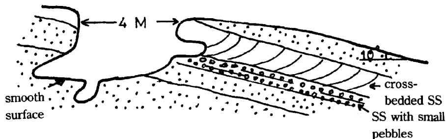
Fig. 14 Replica of Salt Dyke Showing the Former Flowage of Rock Salt, at Tham Kwang, B. Hing Rong, A. Phu Wiang, C. Khon Kaen
