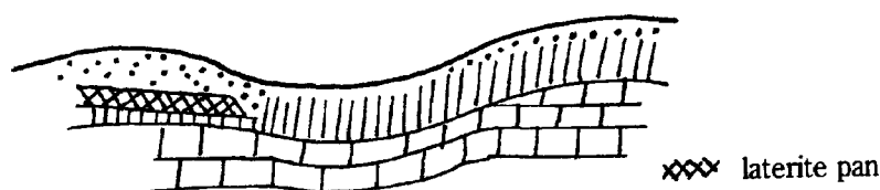
(4) Laterite pan is formed in the lower terrain; iron pisoliths are formed on the crest.
