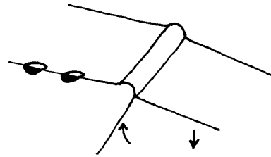
Fig. 22 Sliding and Fracture of Slabs, in Relation with Sinkhole Development (South of Waritchaphum)
