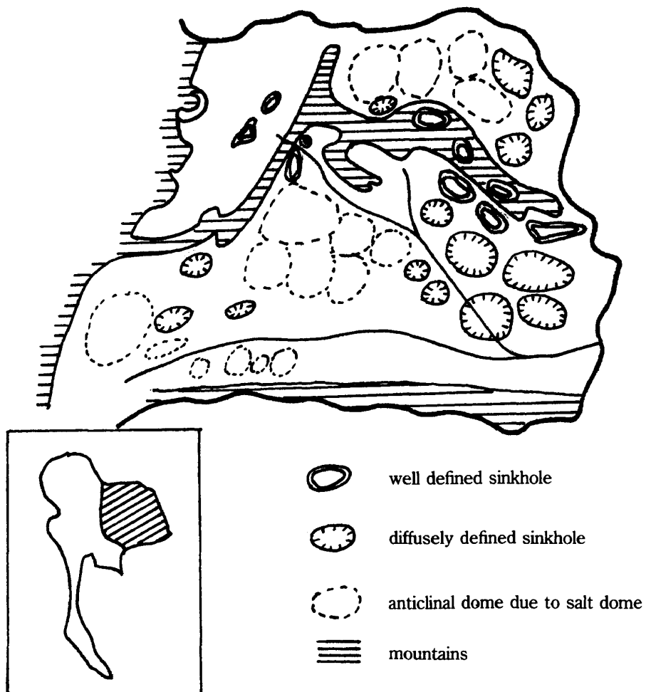
Fig. 17 Schematic Distribution Map of Sinkhole Topography in Khorat Plateau
