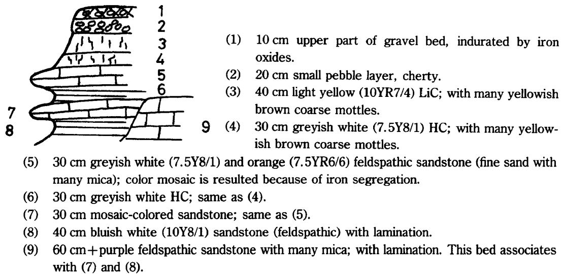
Fig. 11 Vertical Exposure of Differently Altered Saprolite
