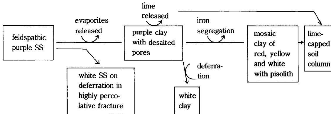
Fig. 9 Alteration of Purple Sandstone into Various Formations
