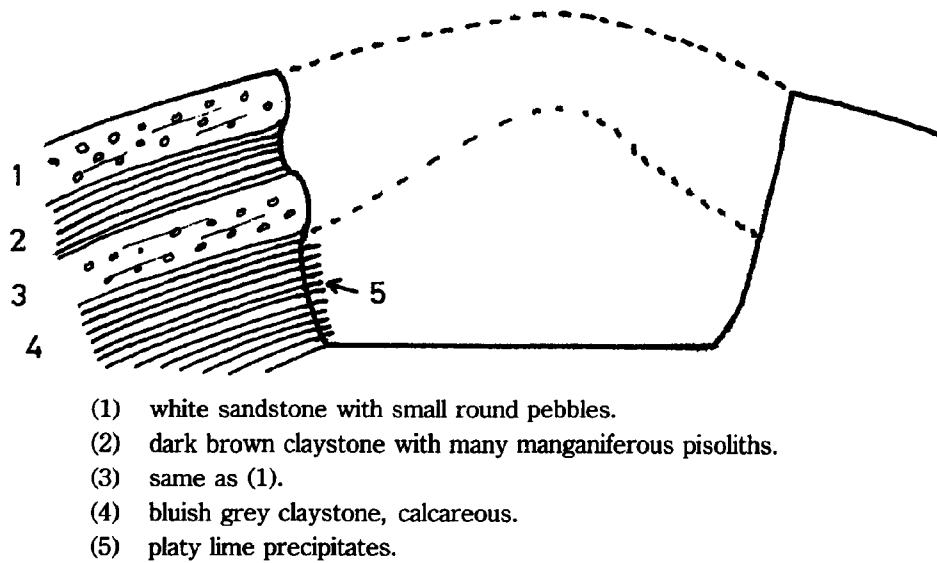
Fig. 15 Schematic Diagram of Khao Wong Sinkhole
