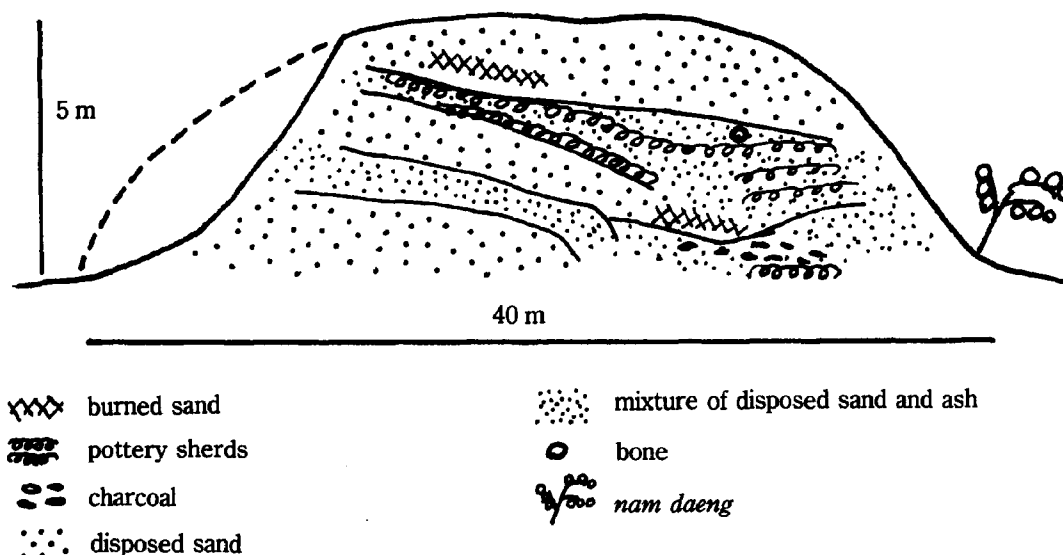
Fig. 3 Exposed Profile of a Salt Mound at B. Nong Suang, A. Non Thai, C. Nakhon Ratchasima
