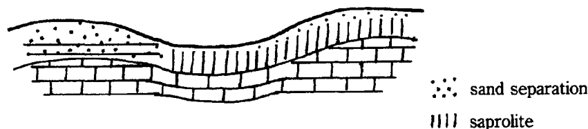
(2) Separation of sand and clay-iron takes place in the feldspathic saprolite; separation of quartz sand takes place in the quartz sandstone.
