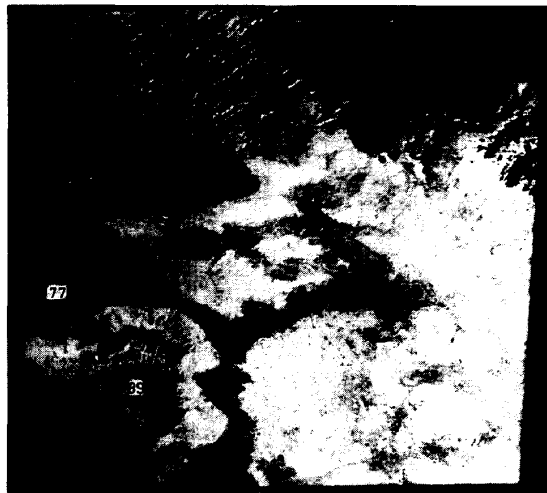
(i) Scene 135-49. 22 Nov. 1975 77. Khemmarat South SH 89. B. Nam SH
