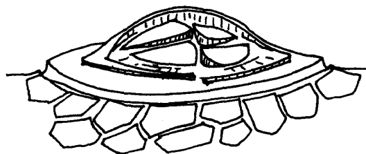
Fig. 20 Mesozoic Nam Dung and Mudcracks at Wat Prabat Phu Phan Khan, C. Khon Kaen near Ubon Rattana Dam
