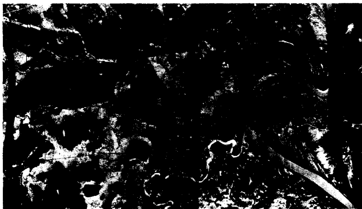
N-S transect at 7 km West of Ubon.
