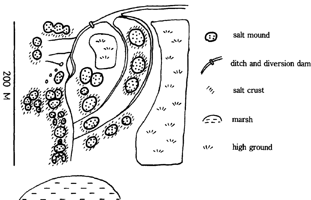
Fig. 2 Arrangement of Salt Mounds and Ditches at B. Khok Sung near Khon Kaen
