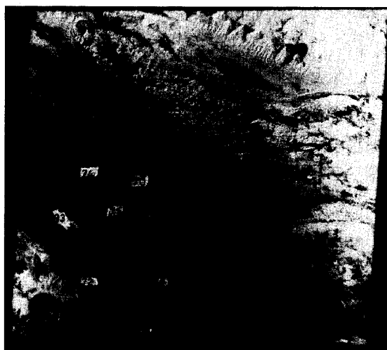
(g) Scene 136-48. 16 Jan. 1976
