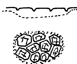
(c) Polygonal mud cracks. Many portions show no reaction with HCl.
