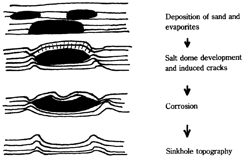
Fig. 13 Schematic Diagram of Phu Wiang Landform
