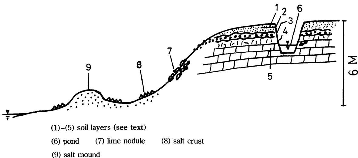
Fig. 4 Fish Pond with Salty Water Located on Hill Crest at B. Khok Sung, Khon Kaen
