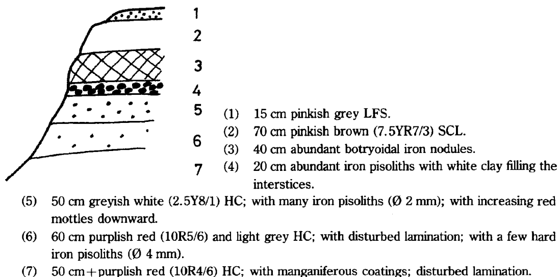
Fig. 10 Vertical Sequence of Alteration Products of Mahasarakham Claystone
