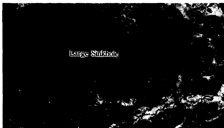
N← (c) Emergence of large sinkhole at more corroded stage.
