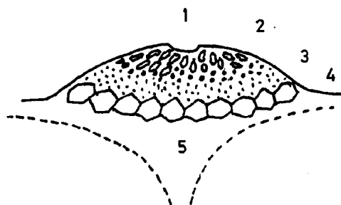
(a) Typical nam dung
