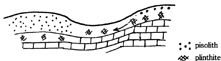
(3) Segregation of clay and iron compounds proceeds; seepage rich in iron compounds flows down along the topography.
