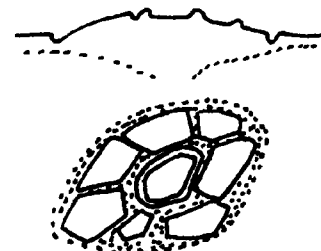
(d) Mud cracks on slightly elevated mound. Sand flow around polygon units.
