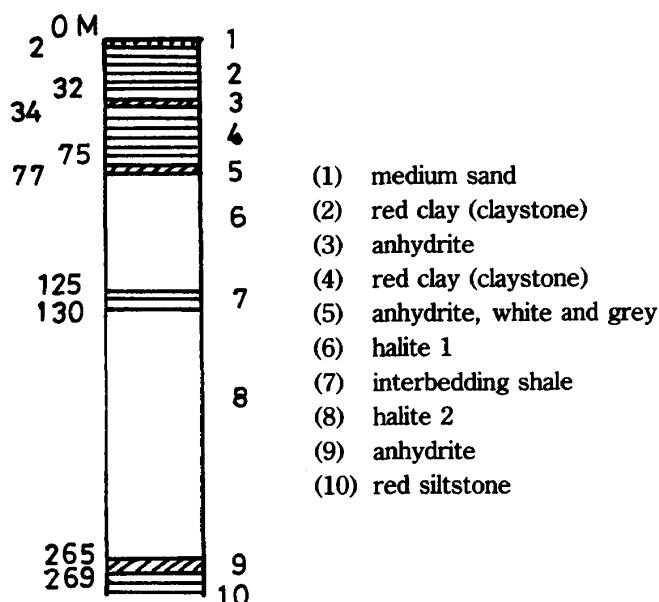
Fig. 5 Drilling Core at Asahi Salt Co., A. Phimai, C. Nakhon Ratchasima
