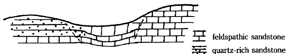
(1) Gentle undulation is formed due to sinkhole topography.
