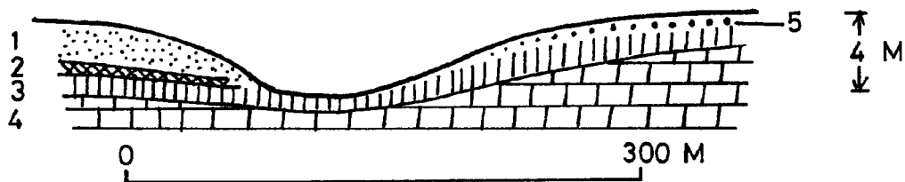
Fig. 25 Control of Soil Properties by bedding Layers
