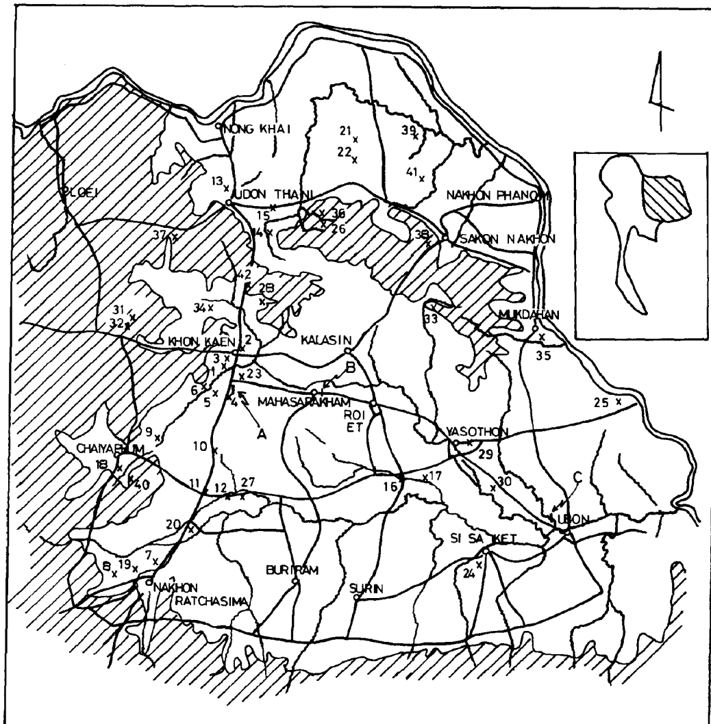
1 B. Khok Sung shown in Fig. 1 & 2. 2 B. Nong Yai 3 B. Si That 4 A. Ban Phai 5 A. Chonnabot 6 A. Mancha Kiri 7 B. Don Kwang 8 B. Nong Suang shown in Fig. 3. 9 A. Khon Sawan 10 A. Ban Phon 11 B. Sida 12 A. Prathai 13 B. Nong Samlong 14 B. Kho Noi 15 A. Nong Han 16 A. Suwannaphum 17 Non Pha Khan 18 B. Nong Na Saeng 19 B. Khok Sung 20 Asahi salt Co. shown in Fig. 5. 21 B. Champadon 22 B. Non Kuam 23 Nam dung site shown in Fig. 6. 24 Outcrop shown in Fig. 7. 25 Outcrop shown in Fig. 8. 26 B. Thung Chuak 27 Outcrop shown in Fig. 10. 28 Outcrop shown in Fig. 11. 29 Outcrop shown in Fig. 12. 30 B. Bung Khrua 31 B. Muang Mai 32 Tham Kwang shown in Fig. 14. 33 Outcrop shown in Fig. 15. 34 Wat Prabat Phu Phan Khan shown in Fig. 20. 35 Outcrop shown in Fig. 21. 36 Outcrop shown in Fig. 22. 37 Wat Tham Khon Pheng shown in Fig. 23. 38 Seri Thai cave in Phu Phan National Park. 39 B. Don Daeng transect shown in Fig. 24. 40 B. Niu transect shown in Fig. 25. 41 B. Na Pho transect shown in Fig. 26. 42 Outcrop shown in Fig. 28. A: Airphoto mosaic shown in Fig. 19(a) B: Airphoto mosaic shown in Fig. 19(b) C: Airphoto mosaic shown in Fig. 19(c)
