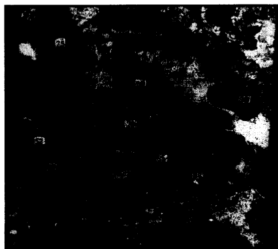
(h) Scene 136-49. 16 Jan. 1976
