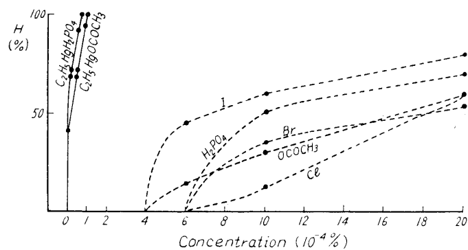
Fig. 1. Relation between H and concentration of various ethyl mercuric compounds (incubation hours : 96 hrs.). — : Inhibiting curve of original solution. --- : Inhibiting curve of solution irradiated for 104 hrs. by weather meter. H : (1 - Cg/C) \times 100\%
