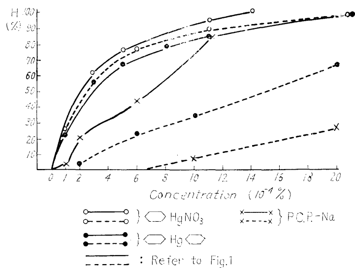
Fig. 4. Relation between H and concentration of phenyl mercuric compounds or P.C.P.-Na.
