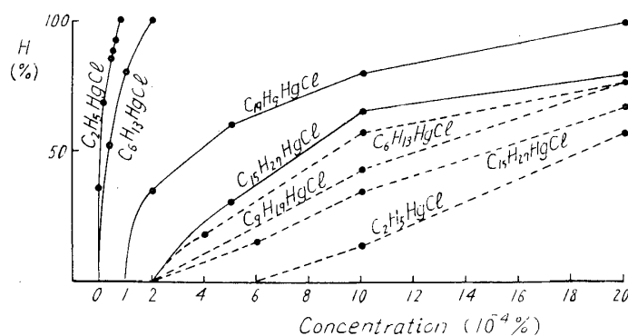
Fig. 2. Relation between H and concentration of various alkyl mercuric chlorides.
