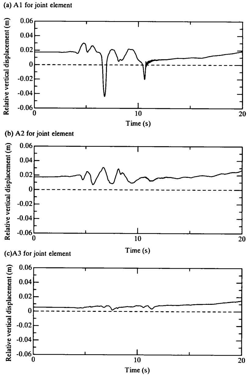
Fig. 6.17 Predicted relative vertical displacements for joint element in Case KB2-1 with M_I=0.48 ( D_r=40\% )
