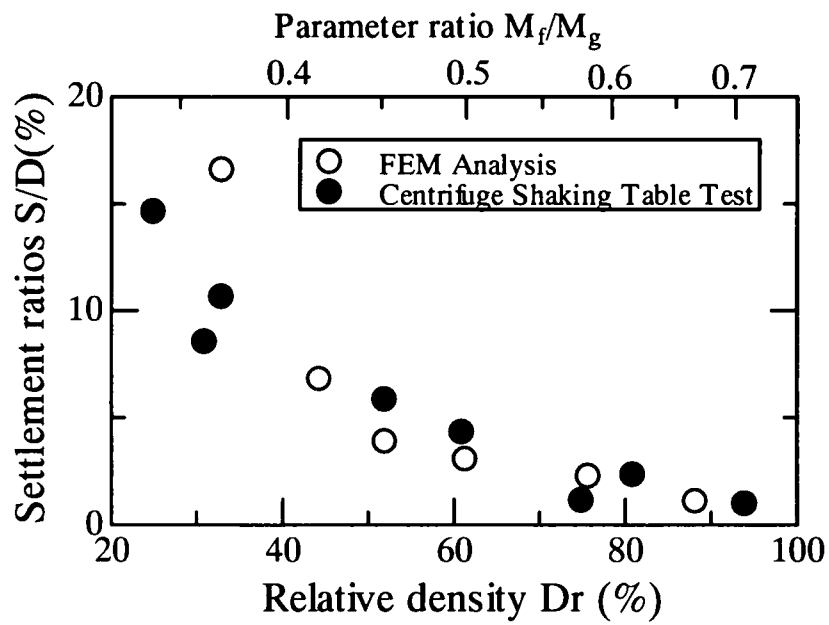
Fig. 5.8 Predicted settlement ratio ( S/D ) plotted against parameter M_r , together with the measured settlement ratio ( S/D ) plotted against the relative density of the foundation soil (after ten cycles of shaking)
