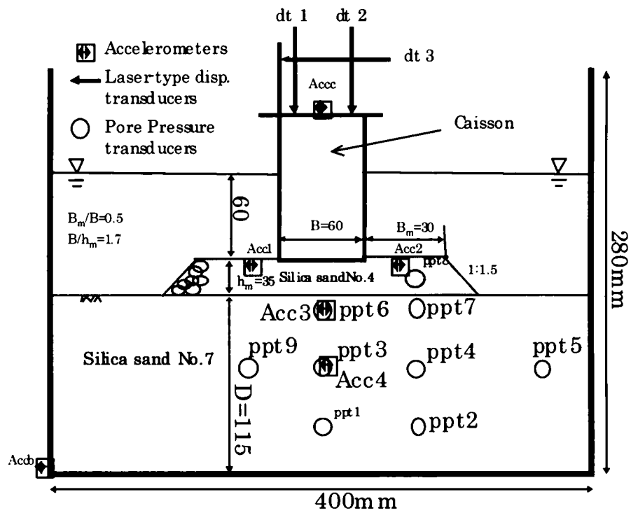
Fig. 5.2 Cross-section of a centrifuge model
