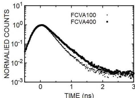
Fig. 1 Lifetime spectra for the DLC samples formed by the FCVA method with different Si bias voltage.
