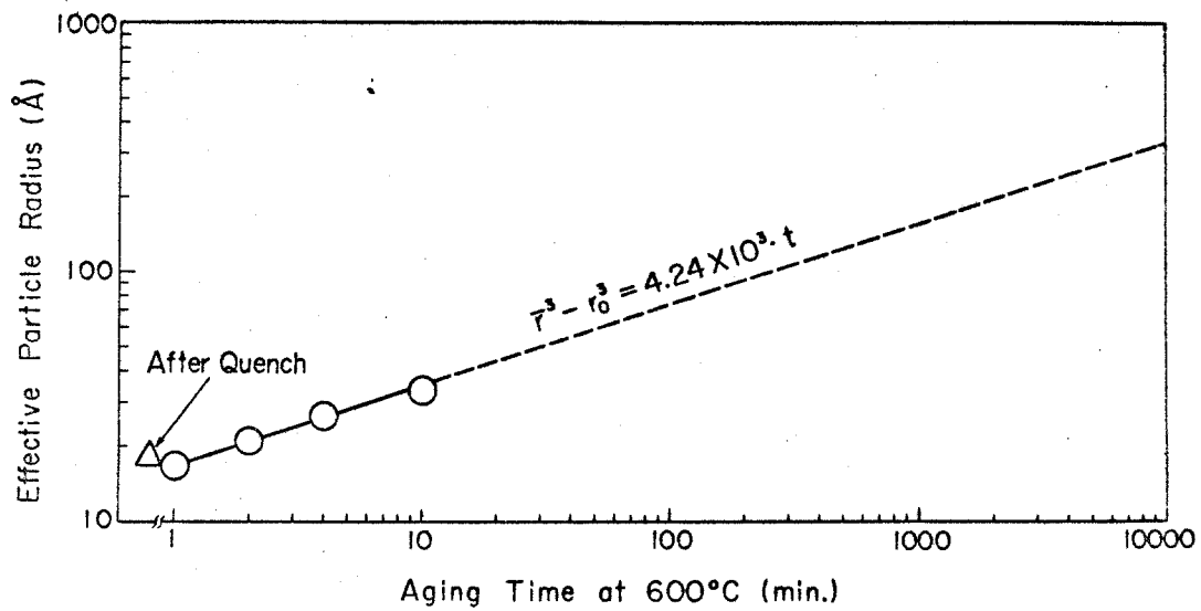
FIG. 42 Change in average precipitated particle size with aging time at 600°C for the Cu-3.52%Co alloy. The straight line was obtained by the extrapolation in Eq. VI-1.
