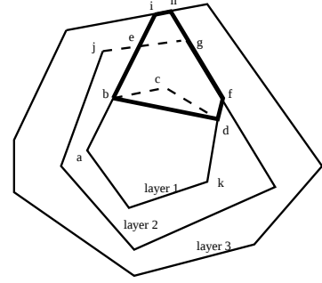
Figure 1: The expansion of a cap bdfhi . The dashed lines represent the removed constraints.
