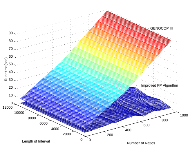
Figure 3: Comparison between GENOCOP III and the 1-D FP algorithm.
