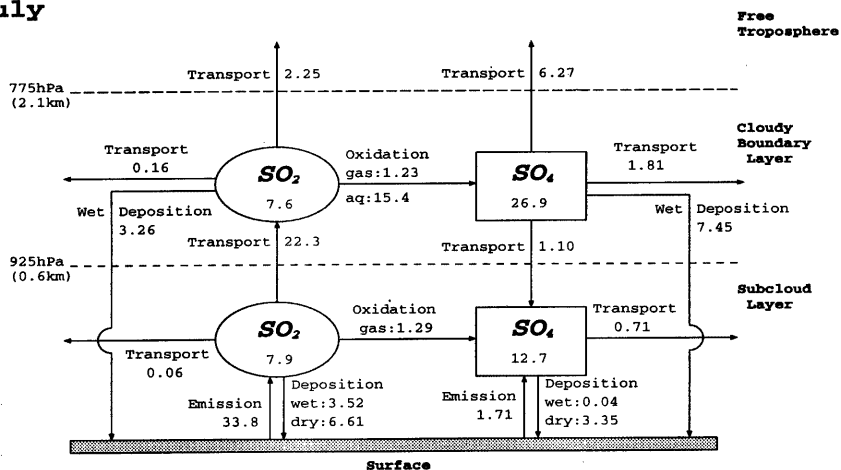
Fig. 4 Monthly regional sulfur budget for 1000 ~ 775hPa column over the United States. Emission flux of SO_2 contains natural source(e.g. oxidation of DMS). Transport flux represents net flux. Unit is GgS for burden, GgS/day for flux.
