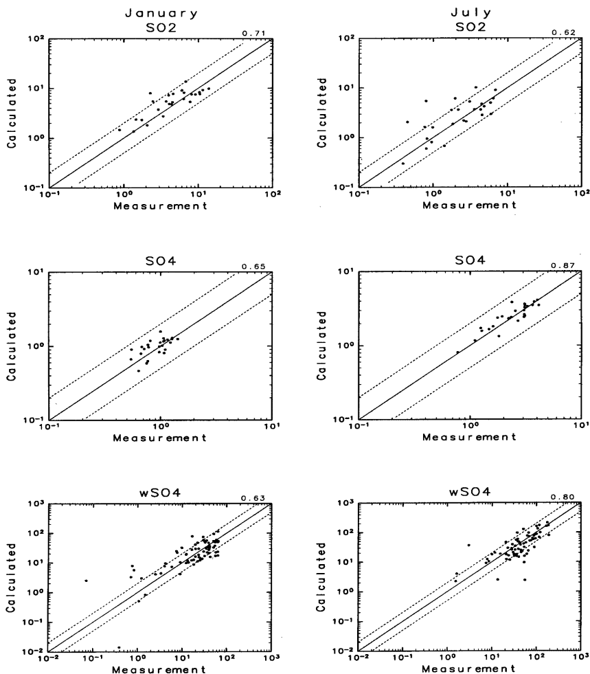
Fig. 3 Comparison between calculation and measurement for North America. Monthly averaged surface SO_2 (unit: \mu g/m^3 ), SO_4 ( \mu g/m^3 ), and monthly SO_4 wet deposition flux ( mg/m^2 ). Three lines represent 1:1 (solid), 1:2 and 2:1 (dashed), respectively. The value at top right is correlation coefficient.
