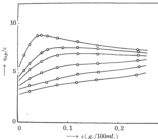
Fig. 8. Observed viscosity curves with \text{MgCl}_2 : The added amounts are, from upper to below, 3.30, 5.67, 10.1, 13.5 and 2.53 ( \text{moles/liter} \times 10^4 ), respectively.
