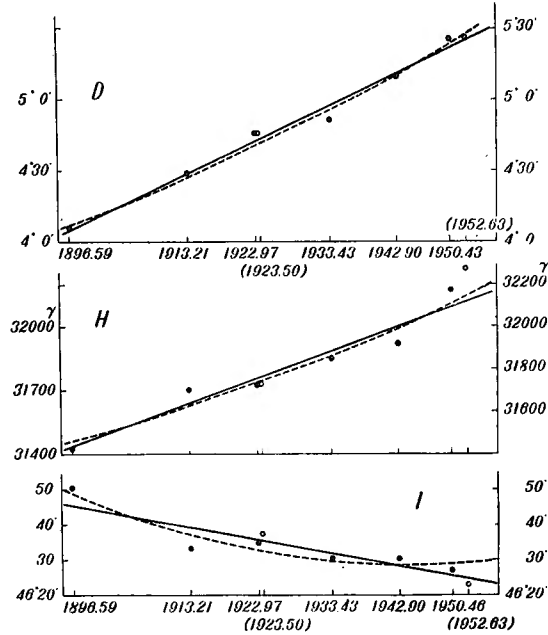
Secular Variation of D, H, and I at the Station No 3 by Hydro. Depart.
