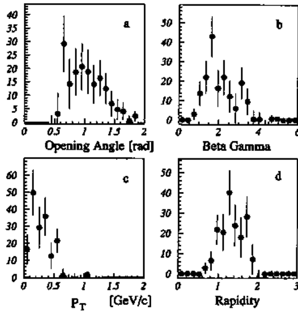
Figure 4.3: The distributions of the opening angle (a), \beta\gamma_{lab} (b), transverse momentum (c), rapidity (d) of the e^+e^- pairs from the carbon and the polyethylene targets. The combinatorial background was already subtracted in the figures.
