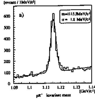
Figure 3.7: Invariant mass spectrum of p\pi^- . The curve was the best fit result with the Gaussian with a linear background. The vertex position were required to be more than 20 mm apart from the target.
