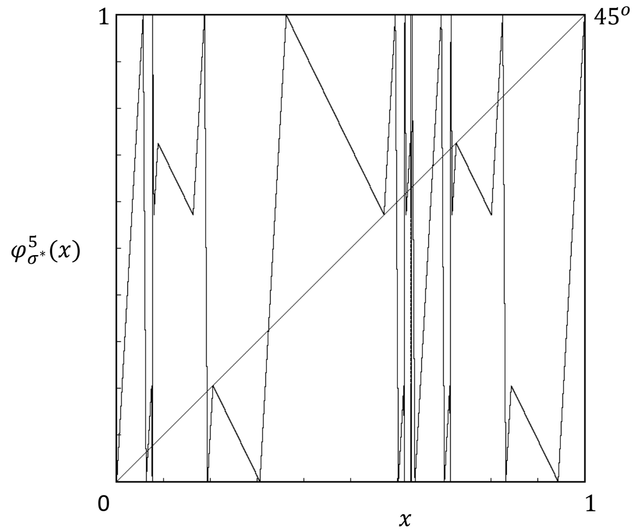
Figure 10: The graph of \varphi_{\sigma^*}^5
