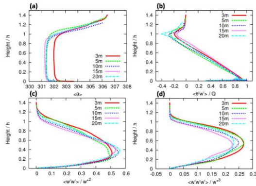
Fig. 2 Vertical profile of horizontally averaged ; (a) potential temperature ; (b) heat flux ; (c) variance ; (d) skewness normalized by the representative parameters.
