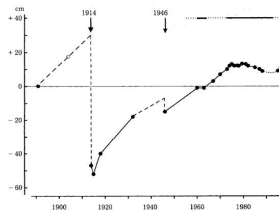
Fig. 6 Vertical ground deformation of the Aira caldera (BM 2474). Arrows indicate large flank eruptions, and horizontal bars do periods of summit eruption
