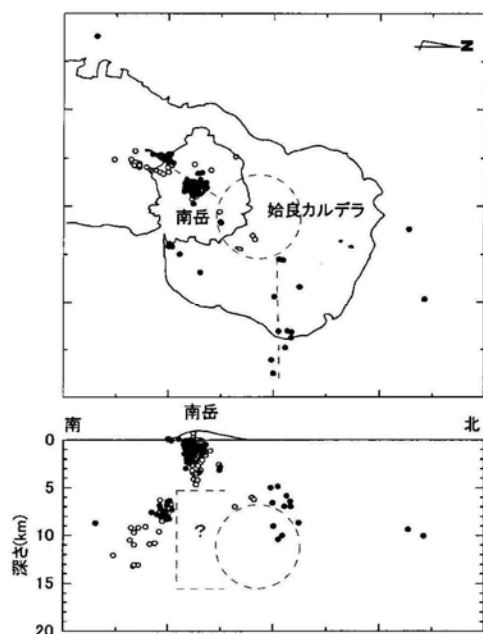
Fig. 8 Distribution of A-type earthquakes (Iguchi, 2006). Open circles indicate those originated before 1988, and closed circles do those during 2001 to 2004.
