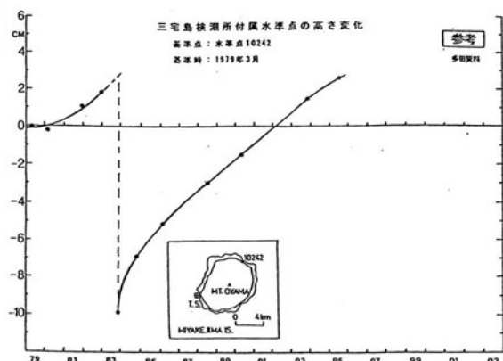
Fig. 4 Vertical displacement at the tidal station south west of Miyakejima referred to BM 10242 (GSI, 1997). The rapid subsidence corresponds to the 1983 eruption.
