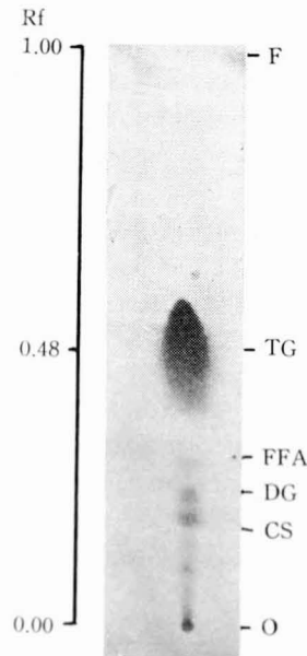
Fig. 2. A typical thin-layer chromatogram of the neutral lipid of C. suppressalis . Sample: from Okayama colony. Solvent system: Petroleum ether/diethyl ether/acetic acid (90:10:1, v/v). See Fig. 1 for detection and abbreviations.
