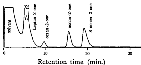
Fig. 3. Gas chromatogram of Fr. 6 in the main attractive fractions.
