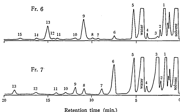
Fig. 6. Gas chromatograms of alcoholic fractions separated from cheese. GLC condition: JGC-750 gas chromatograph (TCD detector), 3mm i. d. \times 2m column packed with 20% PEG-20M on 60-80 mesh celite 545, column temp.; isothermal at 60°C for 5min., then temperature programmed 8°C/min. to 190°C, carrier gas; He 35ml/min., bridge current; 100mA.
