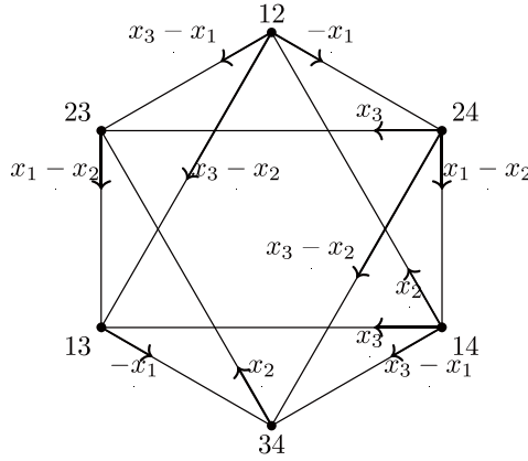
FIGURE 1. The GKM graph (\Gamma_2, \alpha_2) of G_2(\mathbb{C}^4) with T^3 -action.
