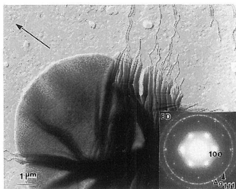
Fig. 7 Granule of PTFE wax L-5 heat-treated on KI at 340^{\circ}\text{C} for 15 minutes and then annealed at 316^{\circ}\text{C} for 1 hour. The arrow indicates the [100] direction of KI and also the direction of Pt-Pd shadowing. The inset is the ED pattern from a plate-like crystal of PTFE (the innermost intense ring is the 111 reflection of Ag).
