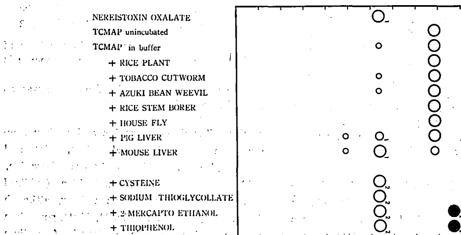
Fig. 3. Paper chromatogram of nereistoxin hydrogen oxalate, TCMAP and its metabolite (reaction products). TCMAP was incubated with homogenates and SH-compounds. Spots were detected by Dragendorff reagent except for black ones, by nitroprusside reagent (1) and by palladium chloride reagent (2).
