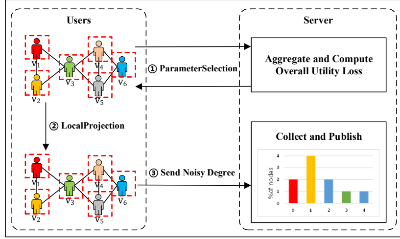
Figure 2.1. Framework of our methods
