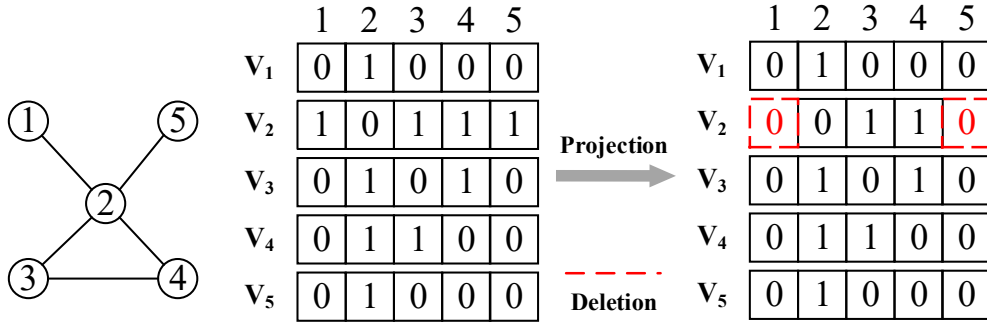
Figure 3.4. Local graph projection. Assume that d'_{max} is equal to 2, user v_2 projects the adjacent bit vector by deleting the edge \langle v_2, v_1 \rangle and edge \langle v_2, v_5 \rangle .
