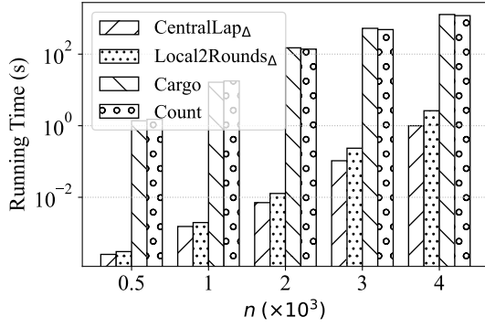
Figure 3.11. Running time on Facebook.
