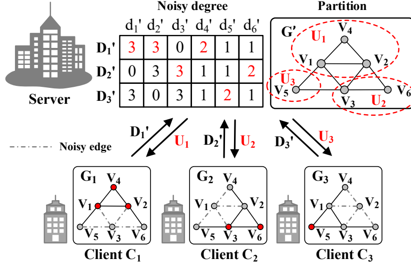
Figure 4.3. Motivation of FEAT+.
