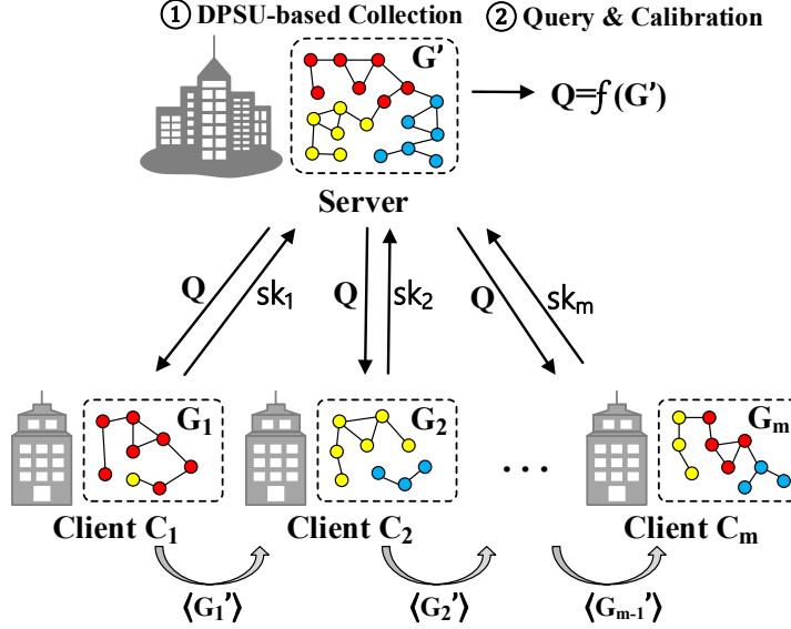
Figure 4.2. Overview of FEAT.
