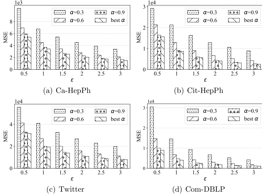
Figure 2.6. The MSE on different graphs, varying \alpha
