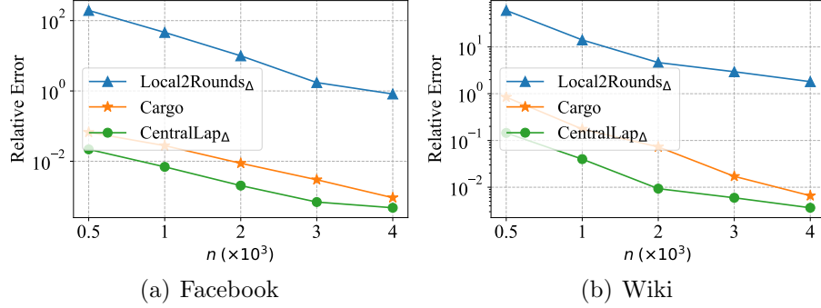
Figure 3.8. The relative error of triangle counting with different n .
