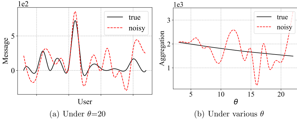
Figure 2.3. The impact of added noise on order information
