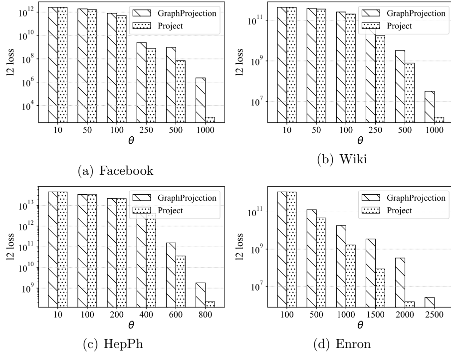
Figure 3.9. The l_2 loss of projection with various parameters.
