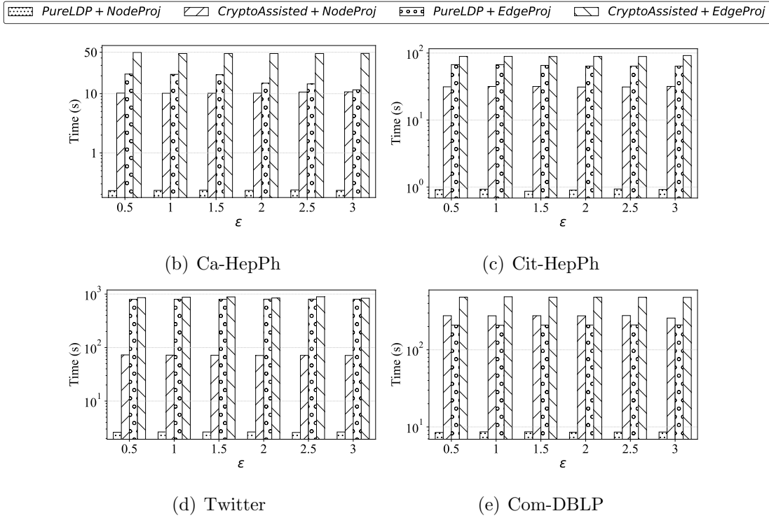
Figure 2.7. The runtime on different graphs
