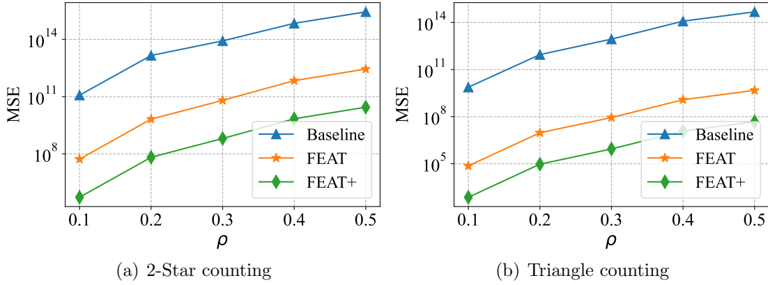
Figure 4.8. The MSE with various \rho .
