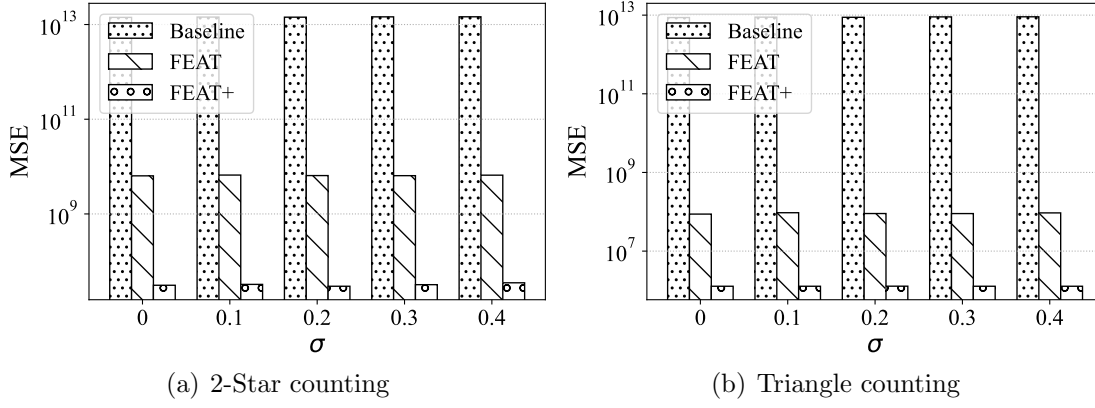
Figure 4.10. The MSE with various \sigma .
