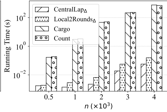
Figure 3.12. Running time on Wiki.
