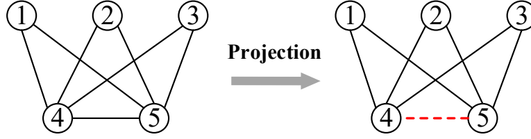
Figure 3.3. Limitation of random deletion. Assume that d'_{max} is equal to 3, if user v_4 (or v_5 ) projects the adjacent list by deleting the edge \langle v_4, v_5 \rangle , all triangles in a graph will be removed.
