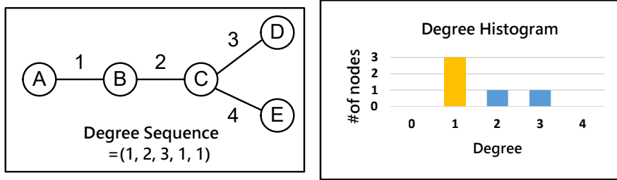
Figure 2.4. Example of degree histogram
