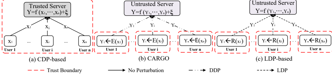
Figure 3.1. A comparison among CDP-based model, LDP-based model and CARGO. (a) CDP-based model relies on a trusted server and achieves a high accuracy, e.g., O(\frac{d_{max}^2}{\epsilon^2}) error; (c) LDP-based model removes a trusted server but introduces more error, i.e., O(\frac{e^\epsilon}{(e^\epsilon-1)^2}(d_{max}^3n + \frac{e^\epsilon}{\epsilon^2}d_{max}^2n)) ; (b) Our CARGO achieves a good utility like CDP-based model, i.e., O(\frac{d_{max}^2}{\epsilon^2}) , but without a trusted server like LDP-based model, where \epsilon, n, d_{max}, d'_{max} denote the privacy budget, number of users, true maximum degree, and noisy maximum degree, respectively.
