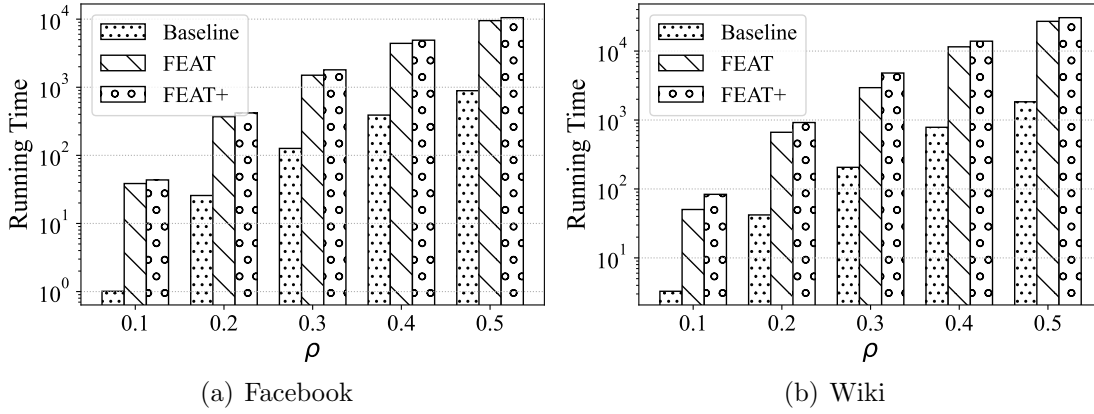
Figure 4.12. Running time with various \rho .
