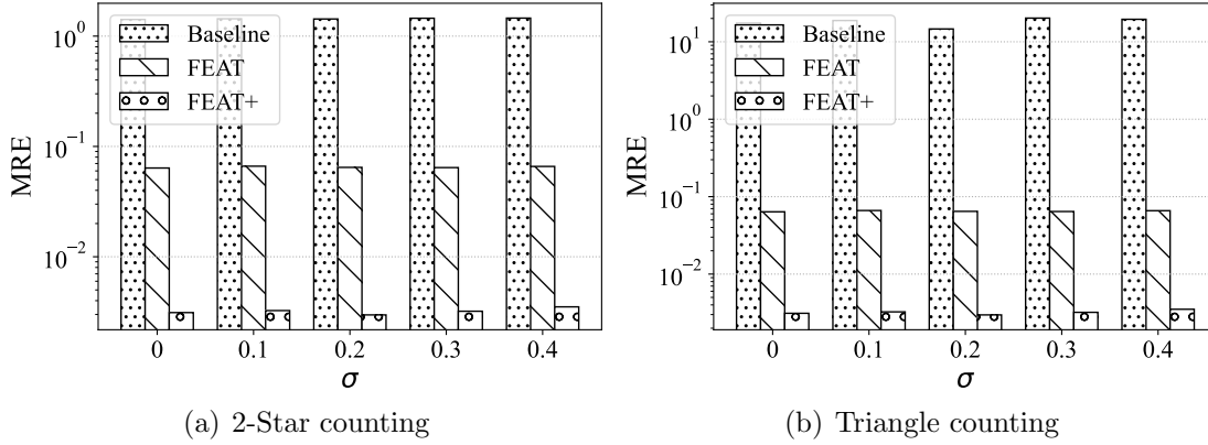
Figure 4.11. The MRE with various \sigma .
