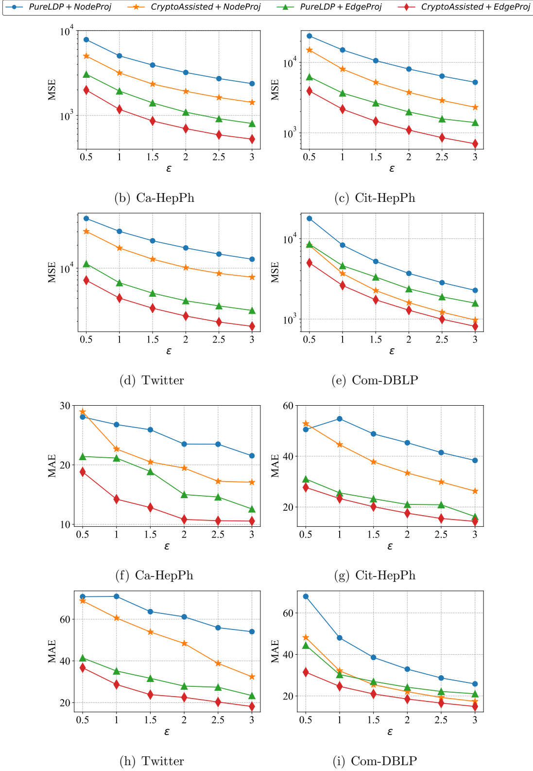
Figure 2.5. The MSE and MAE of algorithms on different graphs
