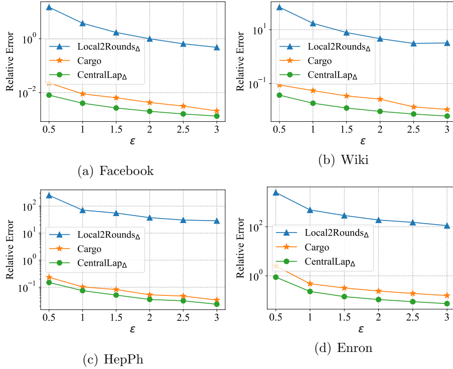
Figure 3.6. The relative error of triangle counting with \epsilon varying from 0.5 to 3.
