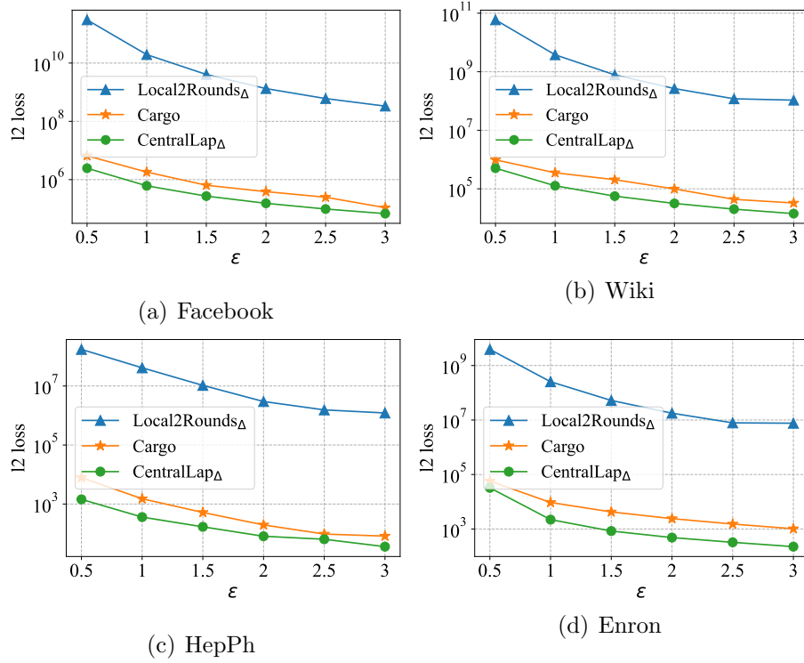
Figure 3.5. The l_2 loss of triangle counting with \epsilon varying from 0.5 to 3.
