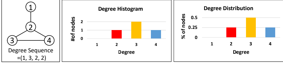
Figure 2.2. Example of publishing degree distribution
