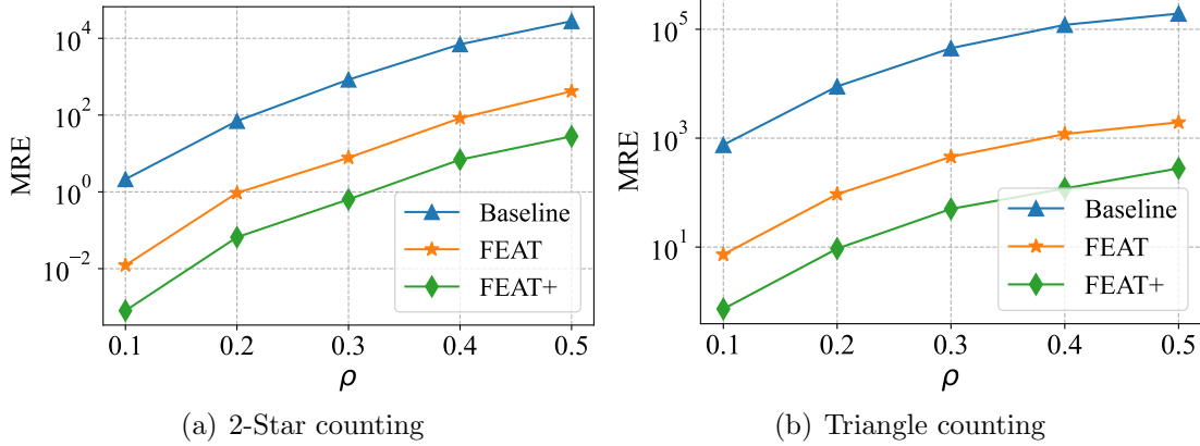
Figure 4.9. The MRE with various \rho .
