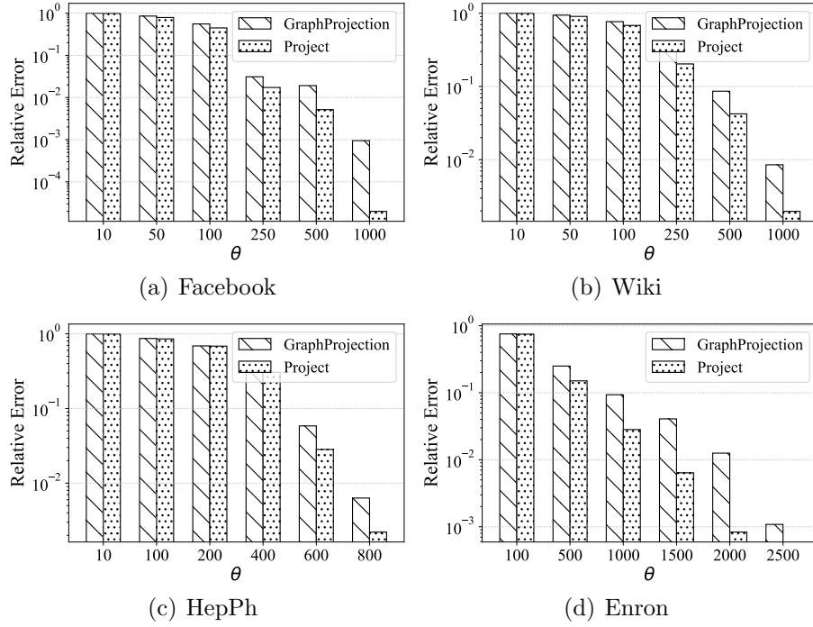
Figure 3.10. The relative error of projection with various parameters.
