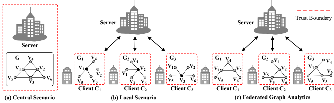
Figure 4.1. Comparisons among central, local and federated scenarios. (a) In a central scenario [1–4], one trusted server owns the entire graph. (b) In a local scenario [5–8], each client owns one node and its 1-hop path information. (c) In a federated scenario, each client owns a subgraph that consists of multiple nodes and edges among them.
