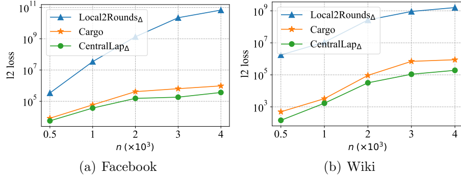
Figure 3.7. The l_2 loss of triangle counting with different n .
