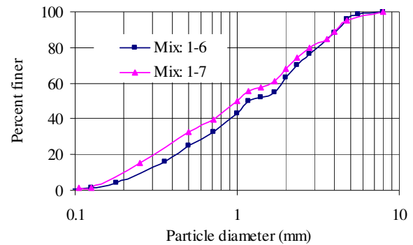
Fig. 5 Grain size distribution of sediment mixes.
