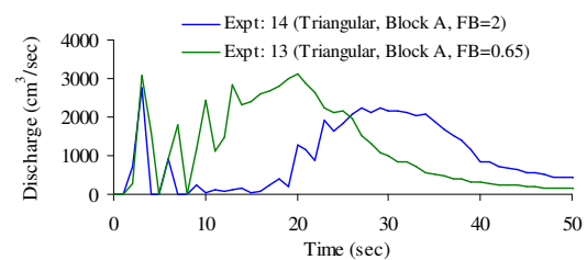
Fig. 14 Outflow hydrographs for dam with different freeboards.
