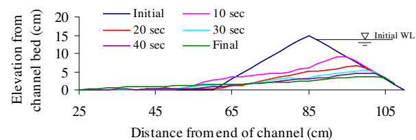
(b) Side channel breach (Expt: 32, Mix: 1-6).
