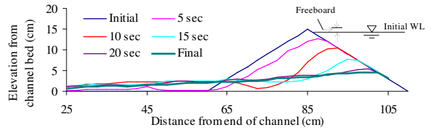
Fig. 13 Dam surface erosion (Expt: 15).
