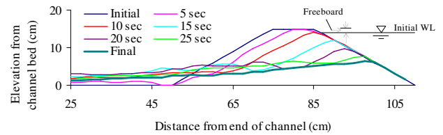
Fig. 12 Dam surface erosion (Expt: 11).
