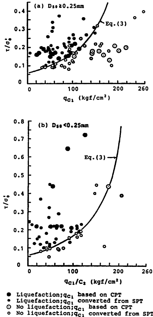
Fig. 2 Correlation between field liquefaction behavior and normalized cone resistance (Shibata & Teparaksa) 10) .
