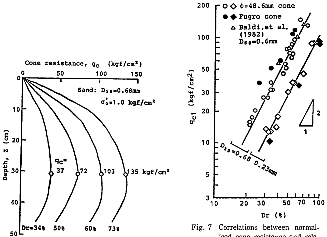
Fig. 6 Example of CPT chamber test.
