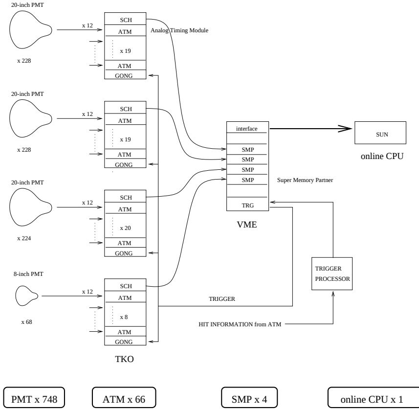
Figure 3.21: The schematic diagram of 1kt data acquisition system.
