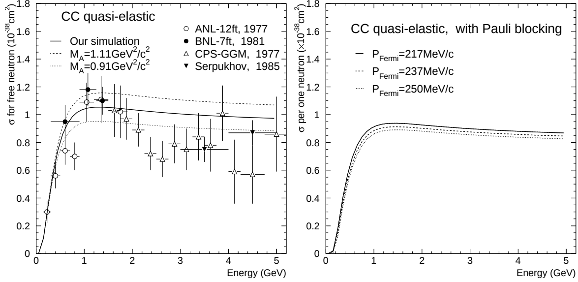
Figure 4.5: (Left figure) Cross section of CC quasi-elastic scattering to one free neutron in our simulation. The standard one with M_A = 1.01 \text{ GeV}^2/c^2 is shown by solid line, whereas the dashed(dotted) line shows the simulation with M_A = 1.11(0.91) \text{ GeV}^2/c^2 . Horizontal axis is the injected neutrino energy in Lab. frame. Measurements from various experiments (ANL:[75], BNL:[76], GGM:[77], and Serpukhov:[78]) are overlaid. Error bars on the marks mean the error quoted in their papers. (Right figure) CC quasi-elastic cross section with Pauli blocking effect. The unit is \text{cm}^2 per one neutron.
