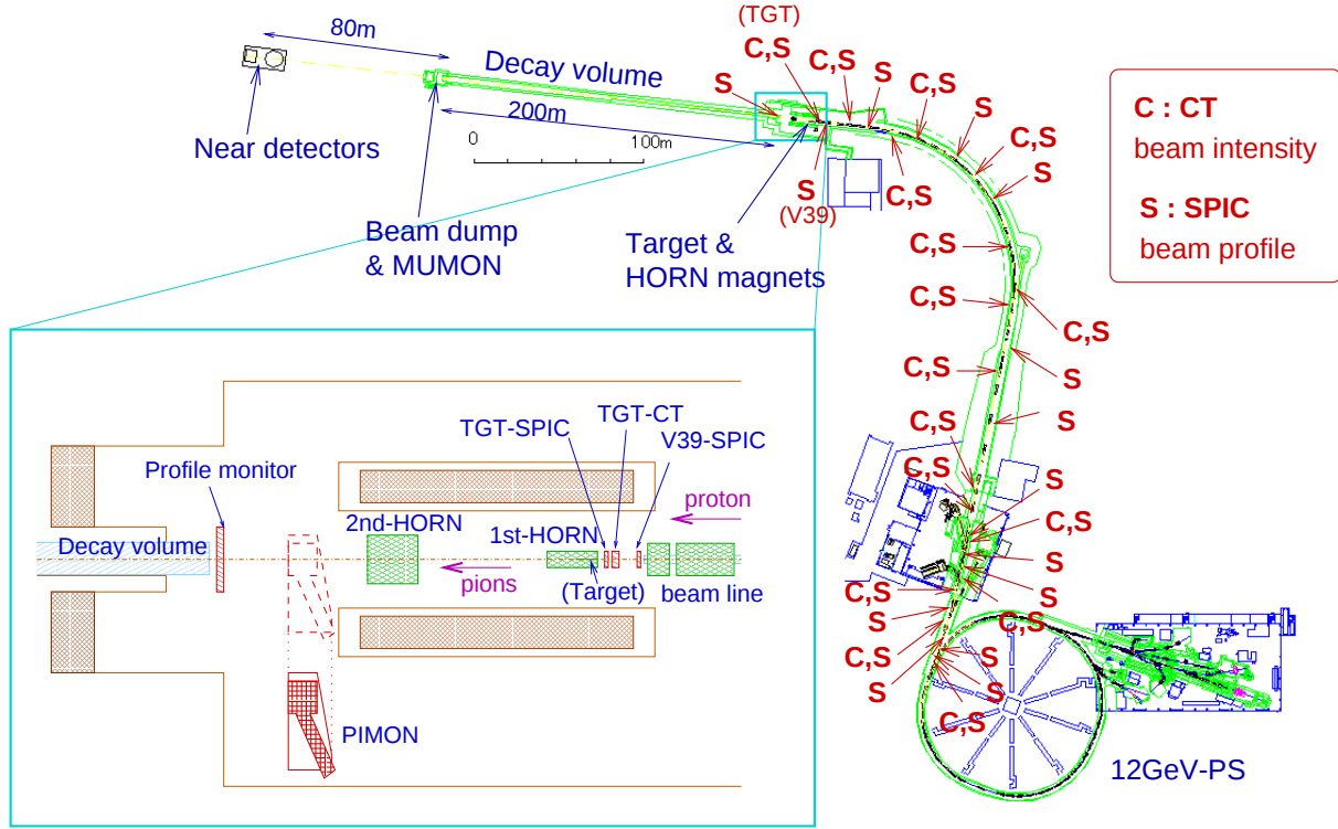
Figure 3.1: Location of the neutrino production beam line components and monitors. Lower-left figure shows a magnification view of the target area.
