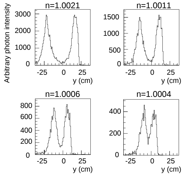
Figure 3.10: Y-directional slice of the typical Cherenkov photon distribution in Monte Carlo simulation, in various refractive indices. Horizontal axis of there figures is the vertical position at the focal plane. Only pions are simulated to emit the Cherenkov photons.
