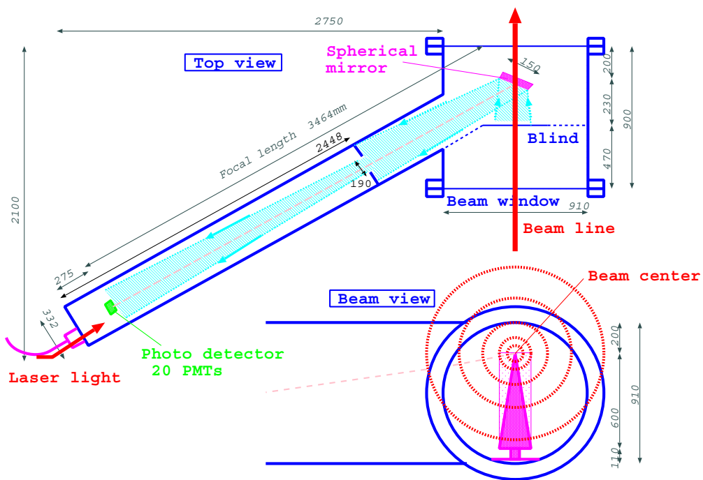
Figure 3.9: The schematic view of PIMON.
