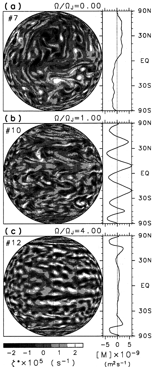
FIG. 5.: Relative vorticity field for the disturbance components (left) and zonal mean zonal angular momentum (right) at t = 1000 J.days for the same three runs as in Fig.4. Map projection is the same as in Fig.1.
