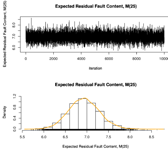
Fig 1 : The MCMC samples and posterior distribution for the expected number of remaining faults at i = 25 , M_{25} .
