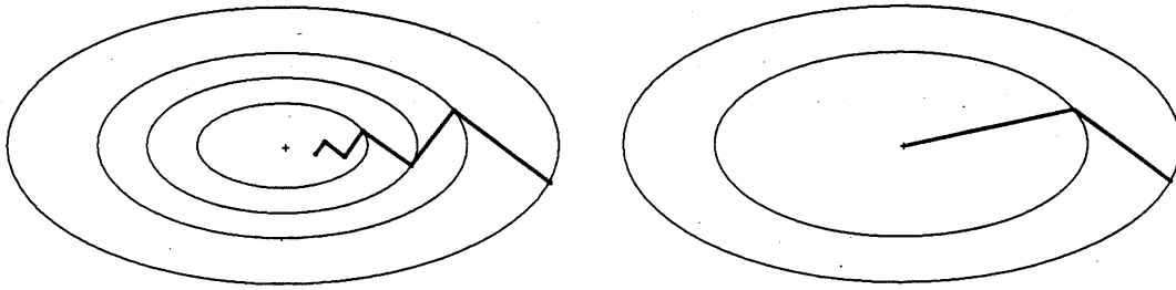
Figure 1: Proceeding of the steepest descent (left) and the classical CG method (right)
