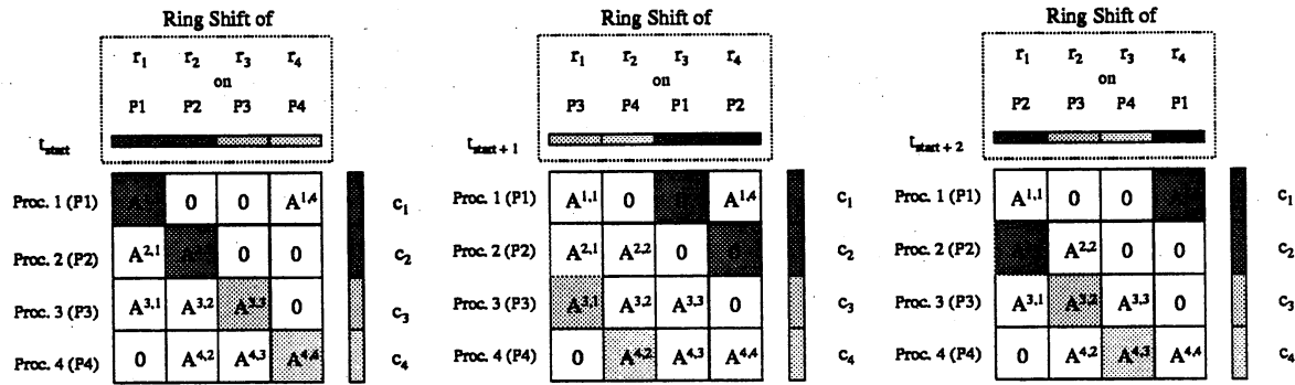
Figure 3: The three computation steps of the matrix-vector multiplication on 4 processors
