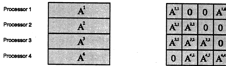
Figure 2: The physical (left) and logical (right) distribution of a matrix to 4 processors
