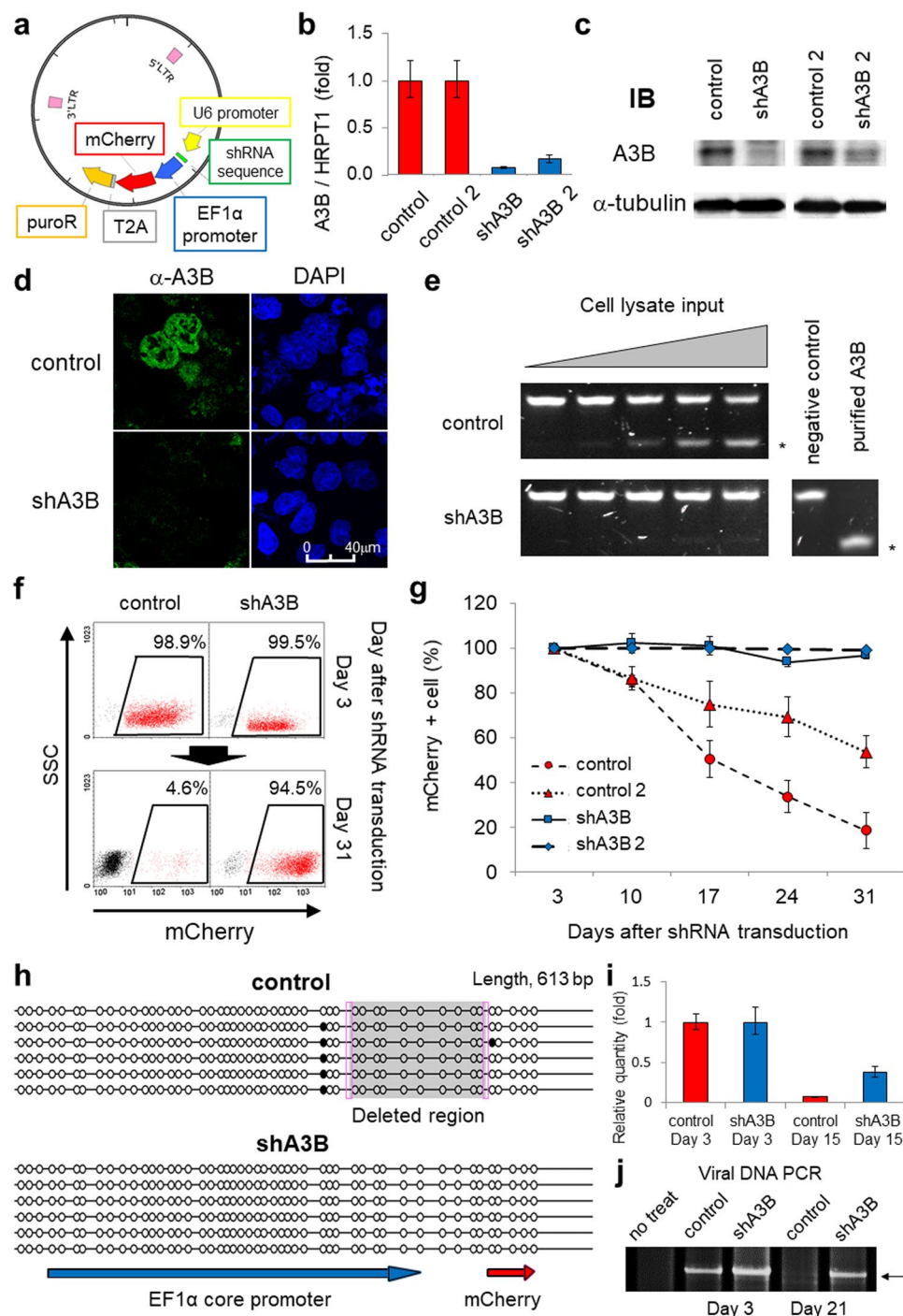
Figure 2. APOBEC3B mediates the loss of function of exogenous genes in myeloma cells. (a) Schema of the shRNA lentiviral vector construct. The produced lentivirus transduces shRNA together with mCherry and the puromycin resistance gene (puroR). (b,c) Real-time PCR (b) and immunoblotting (c) results of A3B levels in RPMI8226 cells, which were transduced with lentiviral shRNA against A3B (two constructs: shA3B and shA3B-2) or control shRNA (two constructs: control and control-2). HPRT1 or \alpha -tubulin was evaluated as an internal control. (d) Immunofluorescence analysis using an anti-A3B antibody of RPMI8226 cells transduced with either shRNA against A3B or control lentivirus. The images were obtained by confocal fluorescence microscopy (magnification, 630x). (e) In vitro assay for cytidine deaminase activity in RPMI8226 cells transduced with either shRNA against A3B or control lentivirus. The asterisks indicate the cleaved DNA products. (f) Flow cytometry of RPMI8226 cells at 3 and 31 days after transduction with each mCherry-shRNA lentivirus. The numbers in boxes indicate the proportions of mCherry-positive cells among the live cells for each condition. (g) Time-dependent changes in the proportions of mCherry-positive cells among live cells transduced with each shRNA lentivirus as determined by flow cytometry. (h) Representative figure of the EF1 \alpha promoter methylation assay. The black circles represent methylated CpG. The shaded box indicates the deleted region. The sense strands of the EF1 \alpha promoter and a portion of the mCherry gene region are shown for reference. The pink boxes indicate
