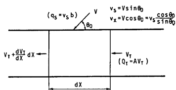
Fig. 2. Flow direction of inflow to vortex tube.
