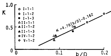
Fig. 7. Relation between coefficient K shown in Fig. 2 and relative slit width b/D
