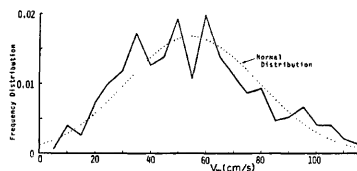
Fig. 9. Frequency distribution of rotating velocity in the vortex tube.
