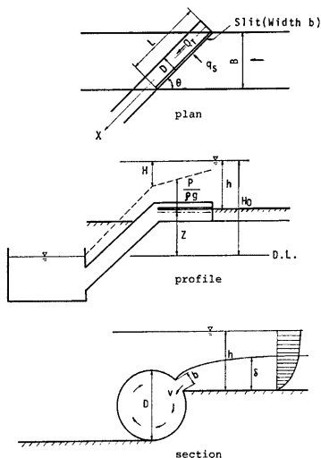
Fig. 1. Vortex tube sand trap — Notation —.
