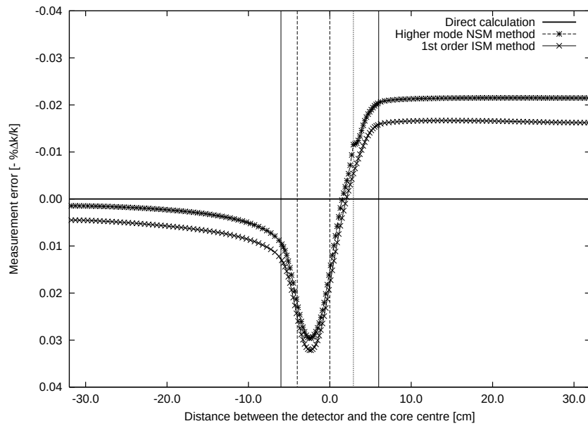
Fig. 3.28 Comparison between the results by two methods, the higher mode source multiplication method and the 1st order imaginary source multiplication method.
