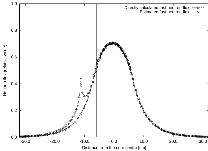
Fig. 3.20 Estimated fast neutron flux distribution by the higher mode source multiplication method for the external neutron source in the reflector region
