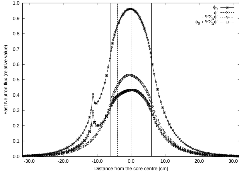
Fig. 3.3 Confirmed agreement of the fast neutron flux distributions. (Solid vertical lines: fuel region, broken lines: region of cross section change, dotted line: the external neutron source.)
