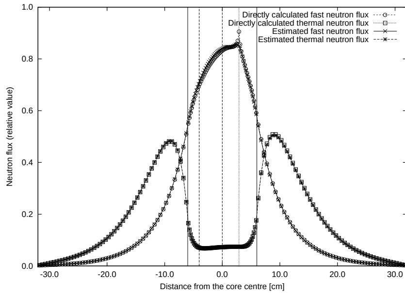
Fig. 3.25 Estimated neutron flux distribution in the case of the local change of cross sections in comparison with the direct calculation.
