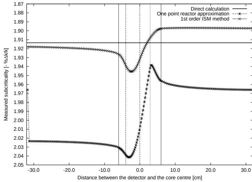
Fig. 3.27 Measurement results by the 1st order imaginary source multiplication method in comparison with those by the one point reactor approximation.
