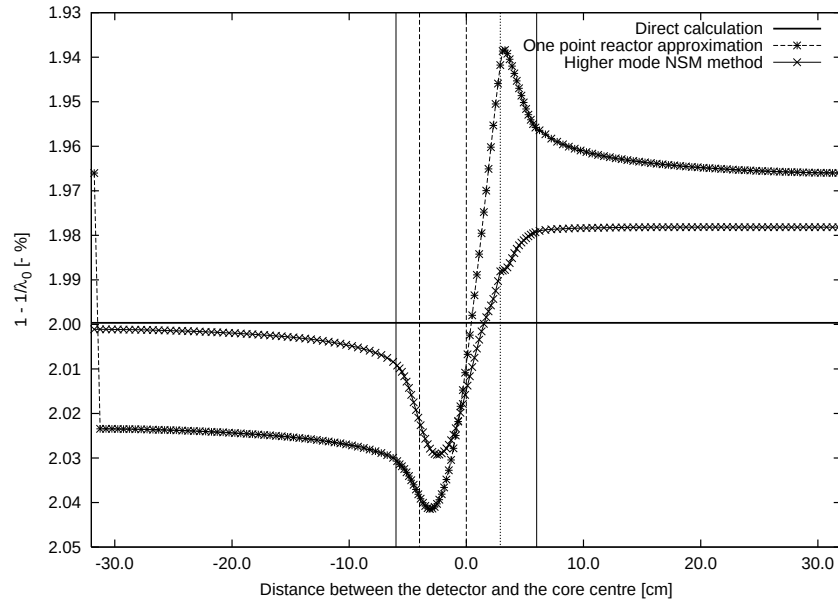
Fig. 3.24 Results of the higher mode source multiplication method for the local change of cross sections. (Solid vertical lines: fuel region, broken: region of cross section change, dotted: the external neutron source.)
