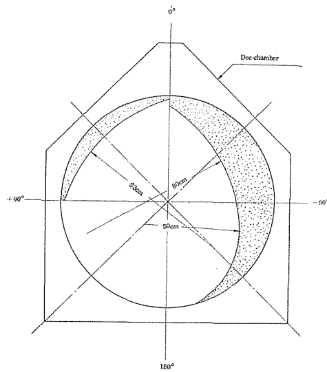
Fig. 8. Shape of the shimming plate. Two semilunar parts which are marked by dots indicate the shape of the shimming plates. The pentagonal frame indicates the dee-chamber.
