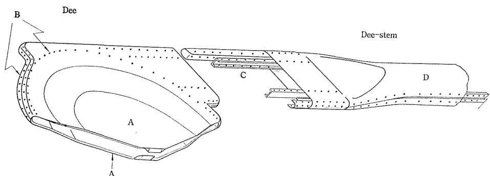
Fig. 13. Illustration of the connection between the dee and the dee-stem.
