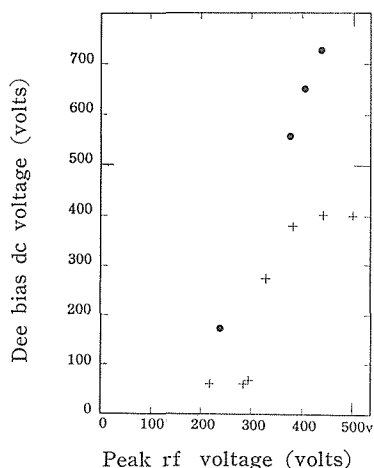
Fig. 16. Voltage necessary to stop the discharge inside the condenser. The crosses and the solid circles indicate the measured values at the pressures of 1 \times 10^{-4} mm Hg and 1.6 \times 10^{-4} mm Hg, respectively.
