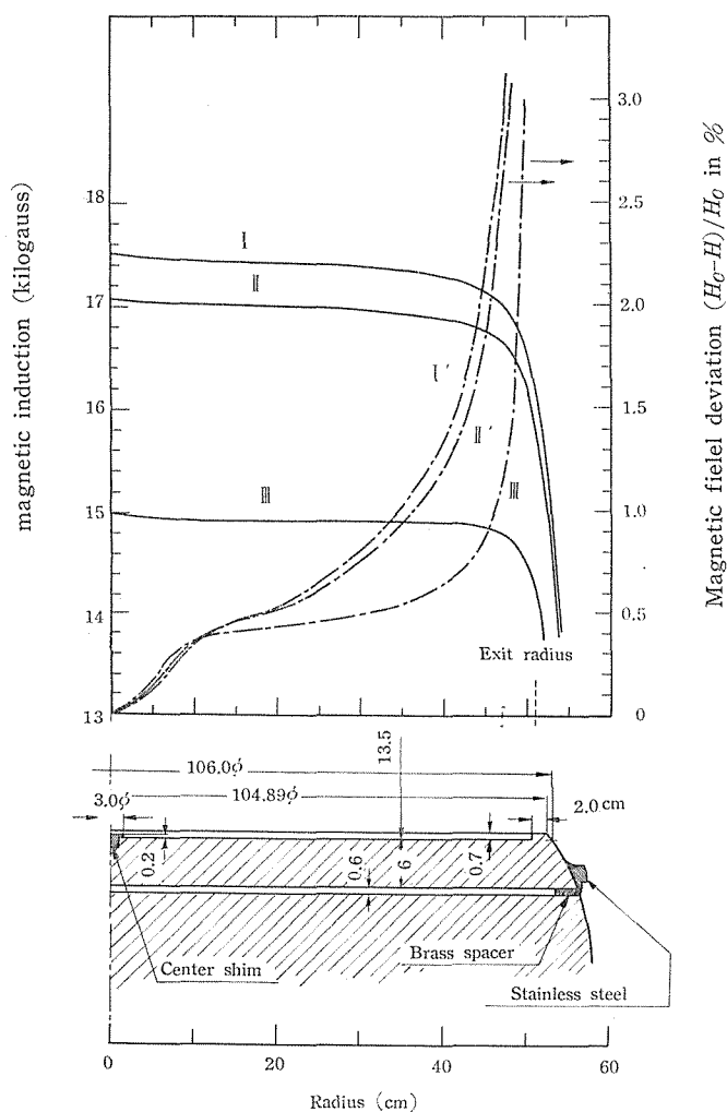
Fig. 6. Radial field distribution of the magnet and the cross-sectional drawing of the pole tip. Curves I, II and III show the radial dependence of the magnetic induction for currents of 138.0, 124.0 and 87.0 amperes, respectively. Curves I', II' and III' show the corresponding magnetic field deviation in percent.
