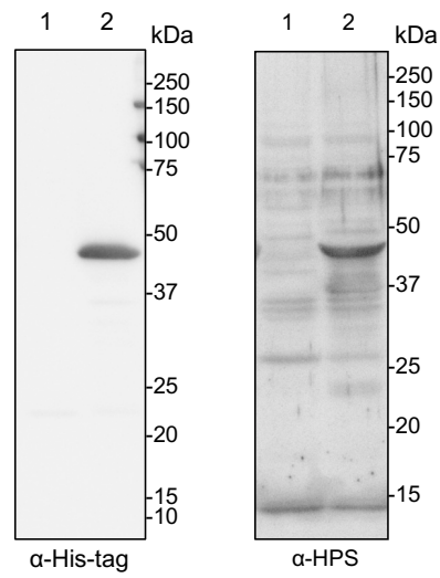
Figure S4. Immunoblot analyses of MDH-His 6 and HPS-PHI proteins in the cell-free extracts of E. coli [pETDuet] (lane 1) and E. coli [pDmHhp] (lane 2) cells. The sizes of the major bands appeared in lane 2 in \alpha -His-tag and \alpha -HPS-detections agreed with that of Fig. S2 and S3, respectively, confirming the co-production of MDH-His 6 and HPS-PHI proteins.
