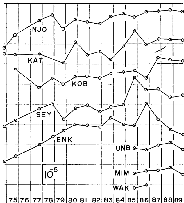
Fig. 11. Accumulation of horizontal strains at base-lines.
