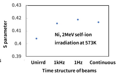
Fig. 2. S-parameter of positron annihilation spectroscopy.
