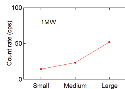
Fig. 2 Count rates of lifetime spectroscopy for different BaF 2 sizes.
