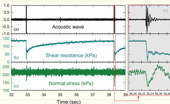
Figure 1. One of selected results for dry granular material sheared under the normal stress about 200kPa and shear velocity of 0.1mm/s. (a) the acoustic wave was recorded in the time domain with the progressive of shearing; (b) the shear resistance; (c) the normal stress; (d) three enlargement figures illustrate the details of acoustic wave, shear resistance and normal stress for the catastrophic failure event (i.e., red boxed-region of the left side), respectively.
