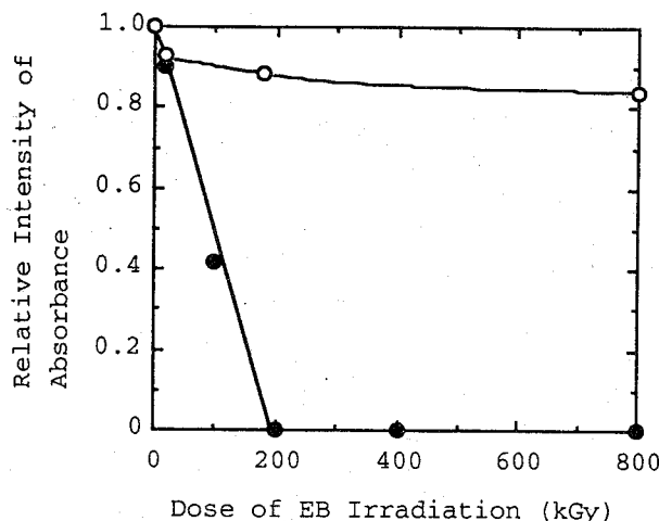
Figure 4. Changes of IR absorption intensities of \nu as(CH 2 ) of CA V-NTS monolayer (●) and ADA LB film (○) of 25 layers as a function of the EB irradiation dose on the basis of the adsorption intensities before EB irradiation.
