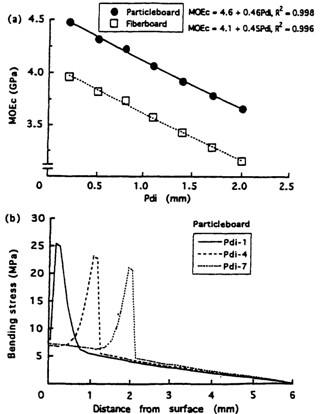
Fig. 3.9. Effect of peak distance (Pdi) on the modulus of elasticity (MOE) (a) and bending stress (b) of particleboard and fiberboard.
