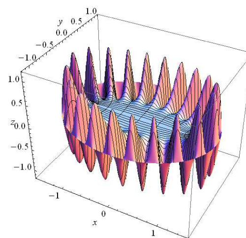
Figure 7. Eigenvalue 344.554.
