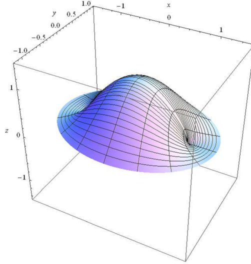
Figure 9. Eigenvalue 3.7379. Imaginary part.
