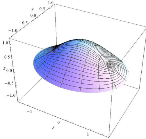
Figure 12. Eigenvalue 3.3944. Graph of v_1 on -\pi \leq \eta \leq \pi .
