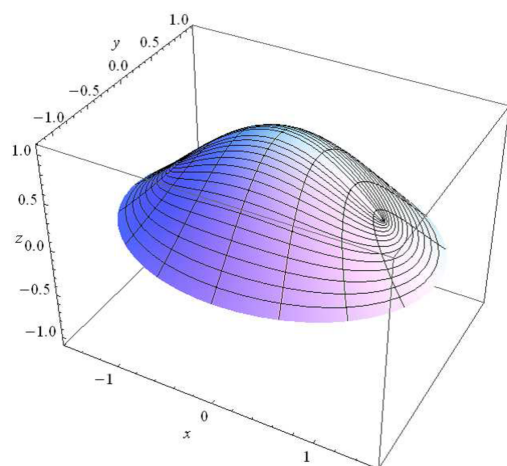
Figure 4. Eigenvalue 3.30141.
