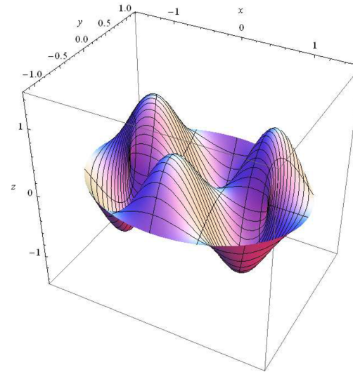
Figure 11. Eigenvalue 20.1521. Imaginary part.
