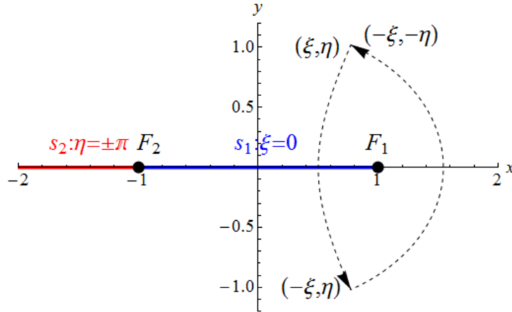
Figure 2. If we vary \xi -coordinate of the elliptic coordinate from \xi to -\xi , and \eta -coordinate from \eta to -\eta subsequently, then the corresponding point turns around F_1 .
