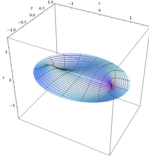
Figure 8. Eigenvalue 3.7379. Real part.
