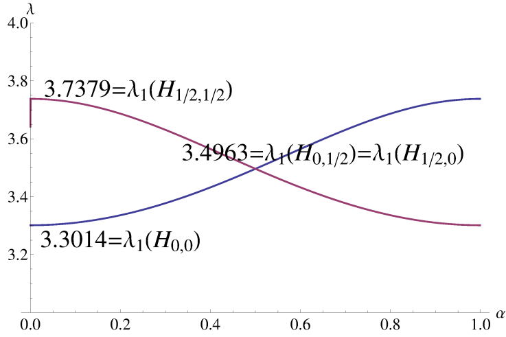
Figure 16. The graphs of the lowest two eigenvalues of -\Delta_{\rho_\alpha} . We see the lowest two eigenvalues of -\Delta_{\rho_\alpha} connect those of H_{0,0} \oplus H_{1/2,1/2} and of H_{1/2,0} \oplus H_{0,1/2} .
