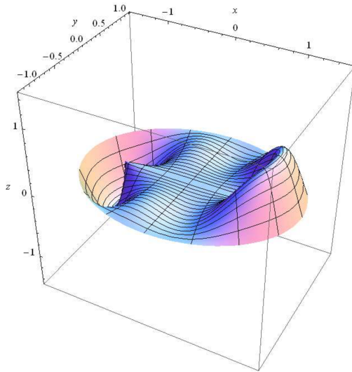
Figure 10. Eigenvalue 20.1521. Real part.
