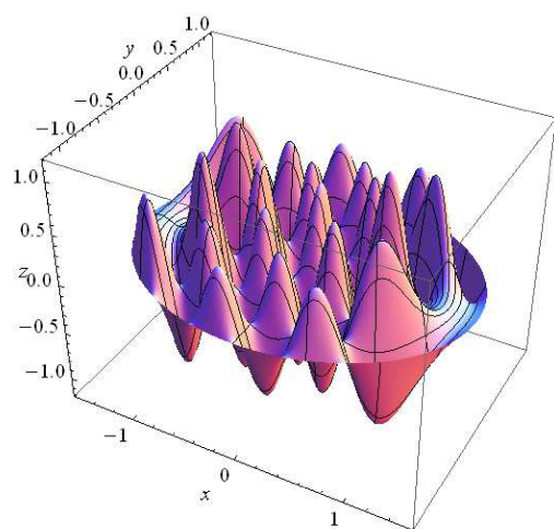
Figure 6. Eigenvalue 187.995.
