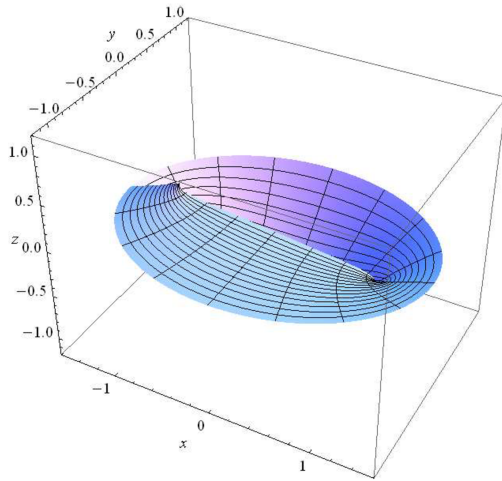
Figure 14. Eigenvalue 3.3944. Graph of v_1 on \pi \leq \eta \leq 3\pi .
