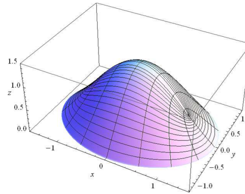
Figure 15. Eigenvalue 3.3944. Graph of v_1^2 + v_2^2 (single-valued).
