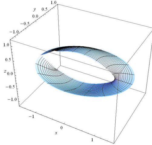
Figure 13. Eigenvalue 3.3944. Graph of v_2 on -\pi \leq \eta \leq \pi .
