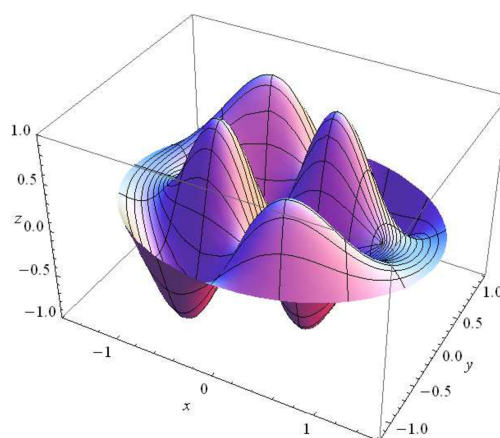
Figure 5. Eigenvalue 42.3785.
