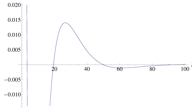
Figure 3. Graph of Ce_0(1, \lambda/4) . The zeros \lambda = 3.30141, 19.4171, 49.9539, 94.7943, \dots are the eigenvalues of the problem (2.1), (2.2).
