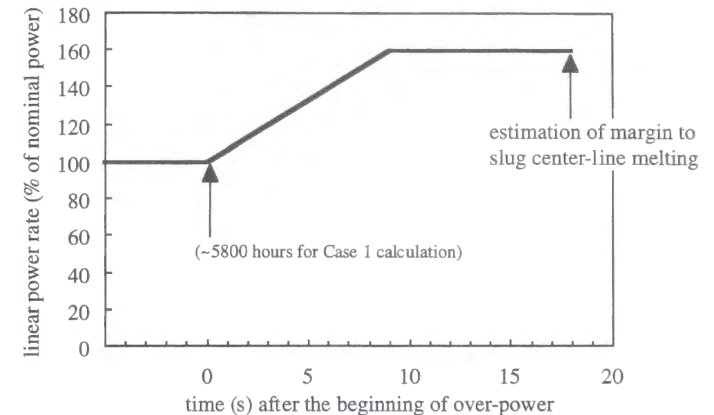
Fig. 3.2.-3 Linear power history for the over-power calculation.
