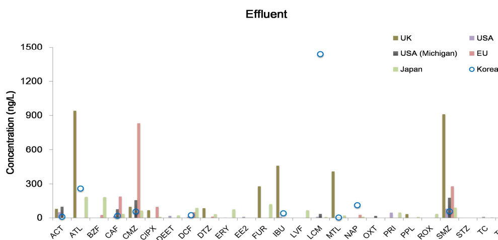
Figure 2.2 Comparison of the concentration of PPCPs and estrogens in effluent from STPs in UK, USA, USA (Michigan), EU and Japan and in Korea
