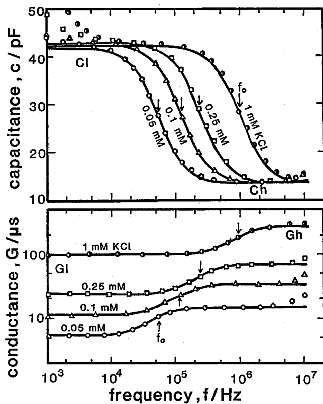
Fig. 5. Frequency dependence of the capacitance C and the conductance G for systems of a 25 hole-film immersed in KCl solutions of 0.05, 0.1, 0.25 and 1 mM. Solid curves are calculated by use of Eqs. 30 and 31.
