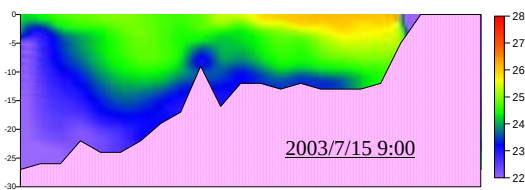
Fig.13 Computation result of the distribution of water temperature along the east-west line in Tanabe Bay
