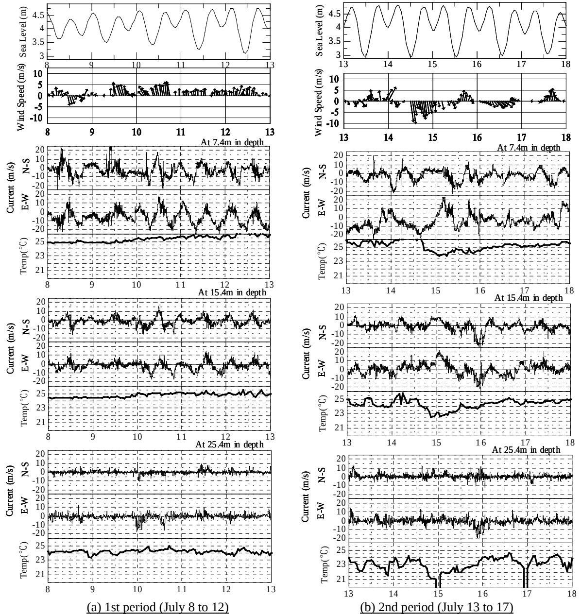
Fig.8 (a) Time series of the tide, wind and current at TNSSOT
