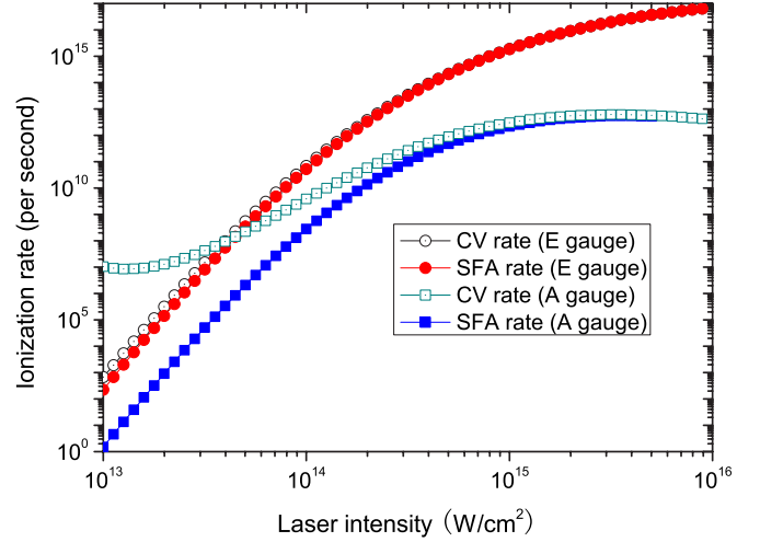
FIG. 4. (Color online) The same as that in Fig. 3, but for a circularly polarized laser field.
