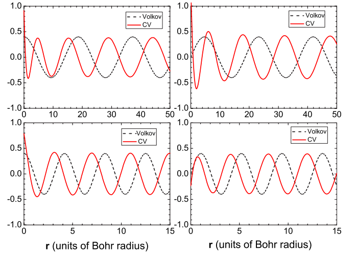
FIG. 1. (Color online) Time-independent parts of the CV (solid line), i.e., u_p^{(-)}(\mathbf{r}) , and Volkov (dashed line) states, i.e., \exp(i\mathbf{p} \cdot \mathbf{r}) , as a function of \mathbf{r} . The energy of electron is chosen to be 1.55 eV (top row) and 31.1 eV (bottom row). The left column is for the real part, and the right column for the imaginary part. We have set \mathbf{p} \cdot \mathbf{r} = pr .
