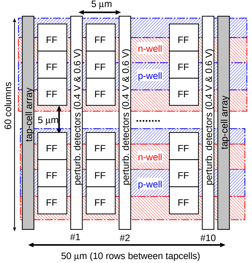
Fig. 2. Block diagram of measurement circuit with detector and shift register.
