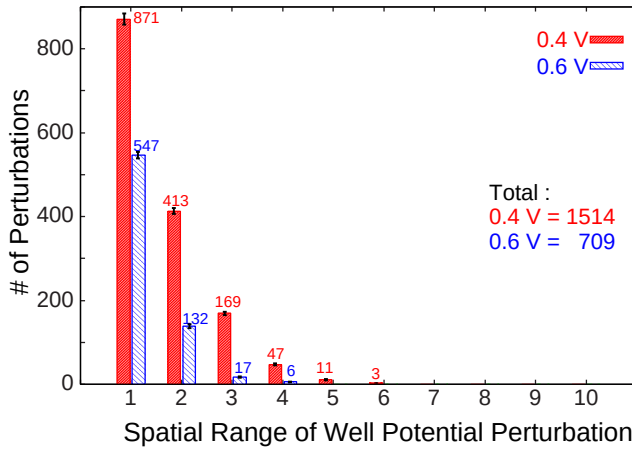
Fig. 8. Spatial range of P-well-potential perturbations.
