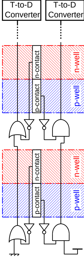
Fig. 1. Well-Potential perturbation detector composed of AND chain, OR chain and two T-to-D converters.
