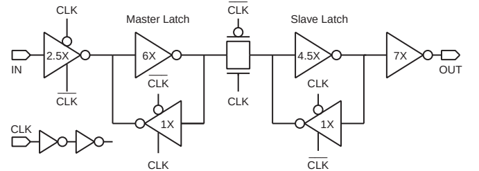
Fig. 3. Schematic diagram of implemented FF.
